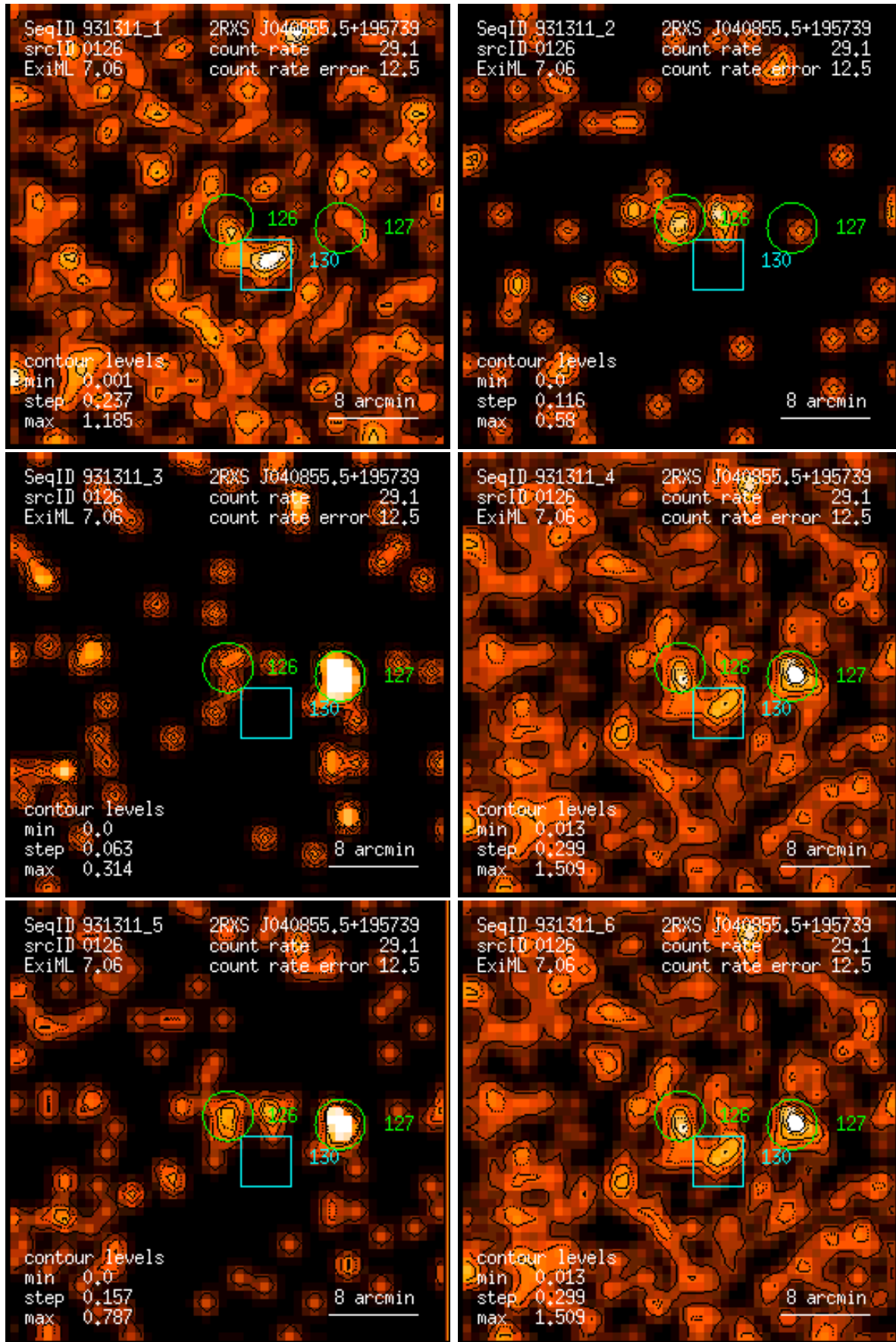
Figure 126: RASS 931311: detection 0126: band rate images, Gaussian filter: (1) PSPC channels 11 – 41, (2) 52 – 90, (3) 91 – 201, (4) 11 – 235, (5) 52 – 201, (6) 11 – 201. Broad band rates in counts/ks. Band rate contour levels in counts/ks/arcmin 2 .
