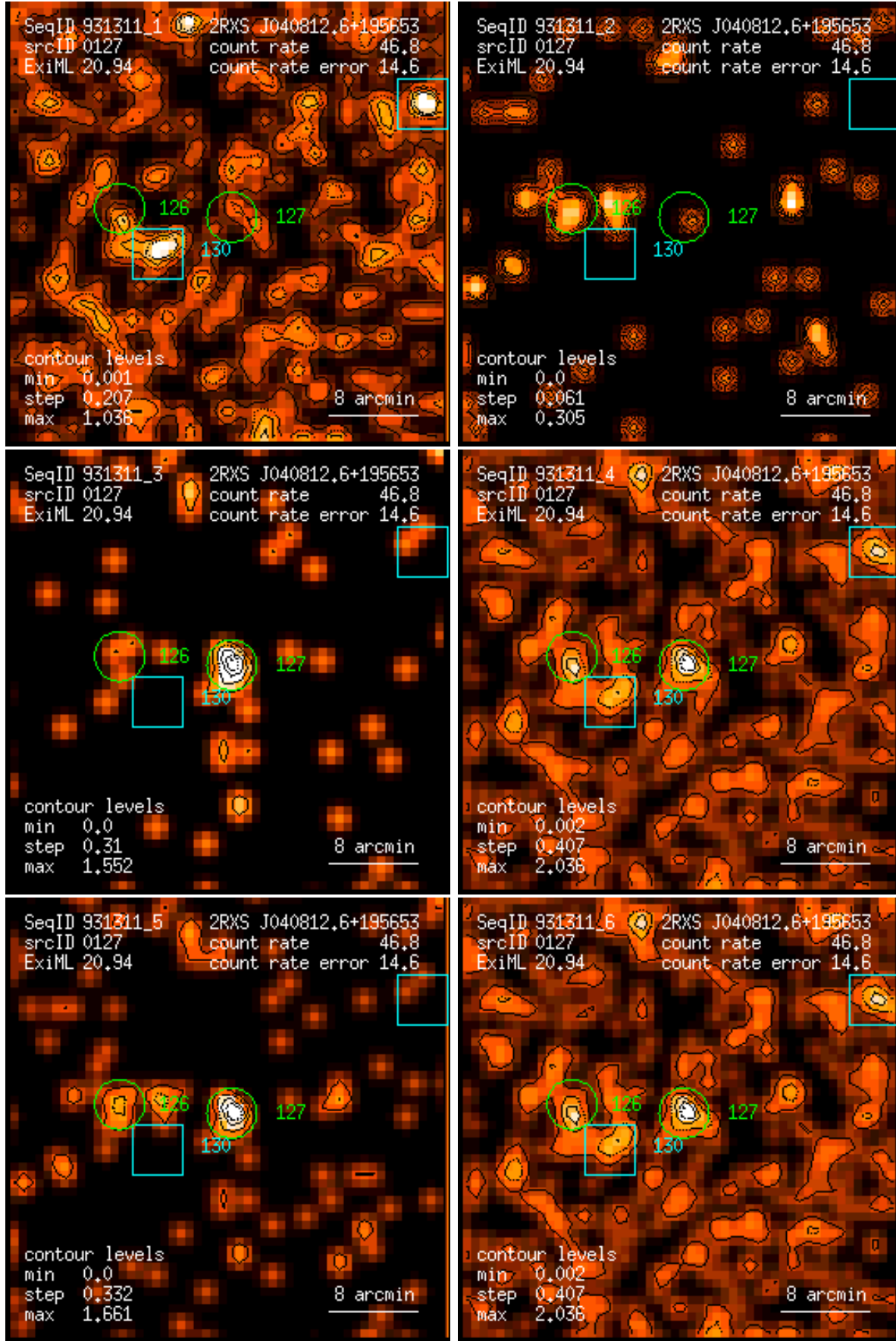
Figure 127: RASS 931311: detection 0127: band rate images, Gaussian filter: (1) PSPC channels 11 – 41, (2) 52 – 90, (3) 91 – 201, (4) 11 – 235, (5) 52 – 201, (6) 11 – 201. Broad band rates in counts/ks. Band rate contour levels in counts/ks/arcmin 2 .
