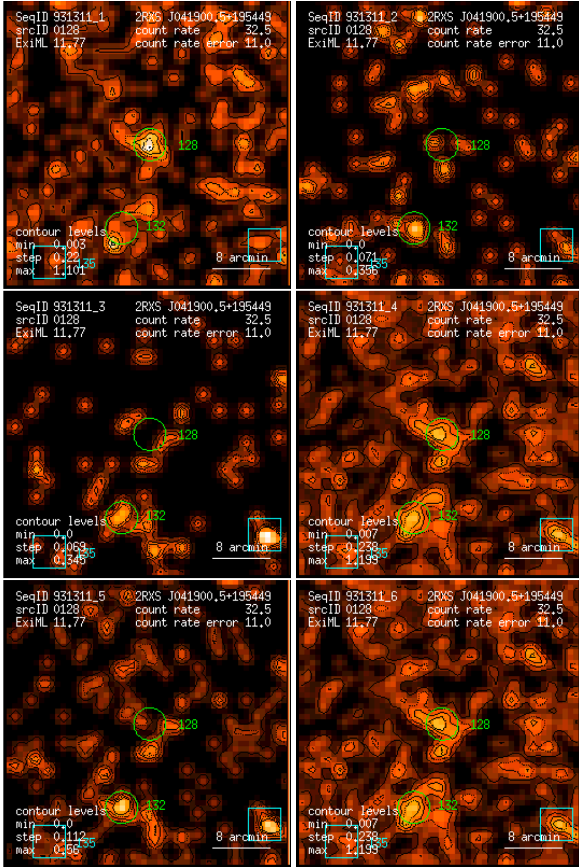
Figure 128: RASS 931311: detection 0128: band rate images, Gaussian filter: (1) PSPC channels 11 – 41, (2) 52 – 90, (3) 91 – 201, (4) 11 – 235, (5) 52 – 201, (6) 11 – 201. Broad band rates in counts/ks. Band rate contour levels in counts/ks/arcmin 2 .
