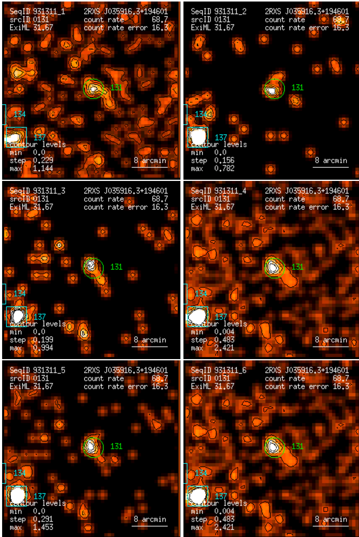
Figure 131: RASS 931311: detection 0131: band rate images, Gaussian filter: (1) PSPC channels 11 – 41, (2) 52 – 90, (3) 91 – 201, (4) 11 – 235, (5) 52 – 201, (6) 11 – 201. Broad band rates in counts/ks. Band rate contour levels in counts/ks/arcmin 2 .
