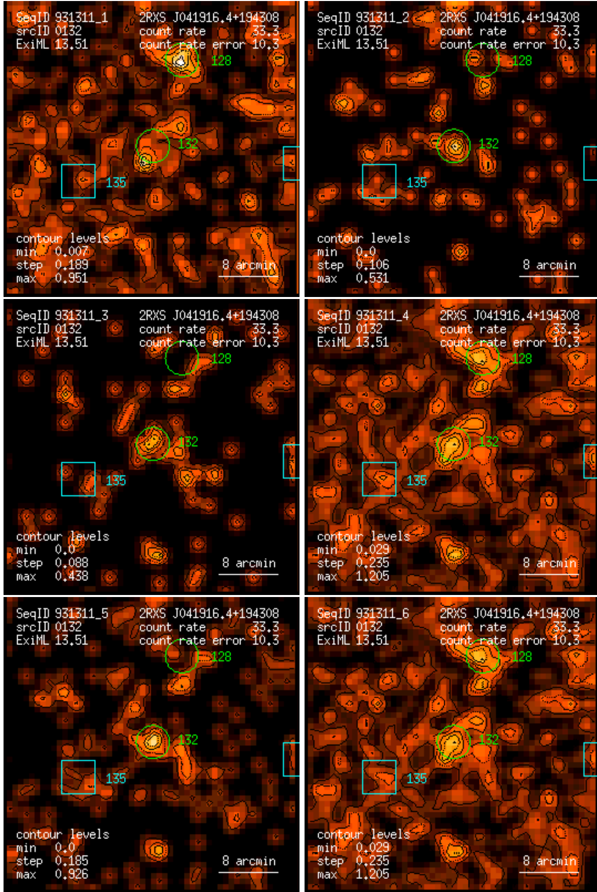
Figure 132: RASS 931311: detection 0132: band rate images, Gaussian filter: (1) PSPC channels 11 – 41, (2) 52 – 90, (3) 91 – 201, (4) 11 – 235, (5) 52 – 201, (6) 11 – 201. Broad band rates in counts/ks. Band rate contour levels in counts/ks/arcmin 2 .
