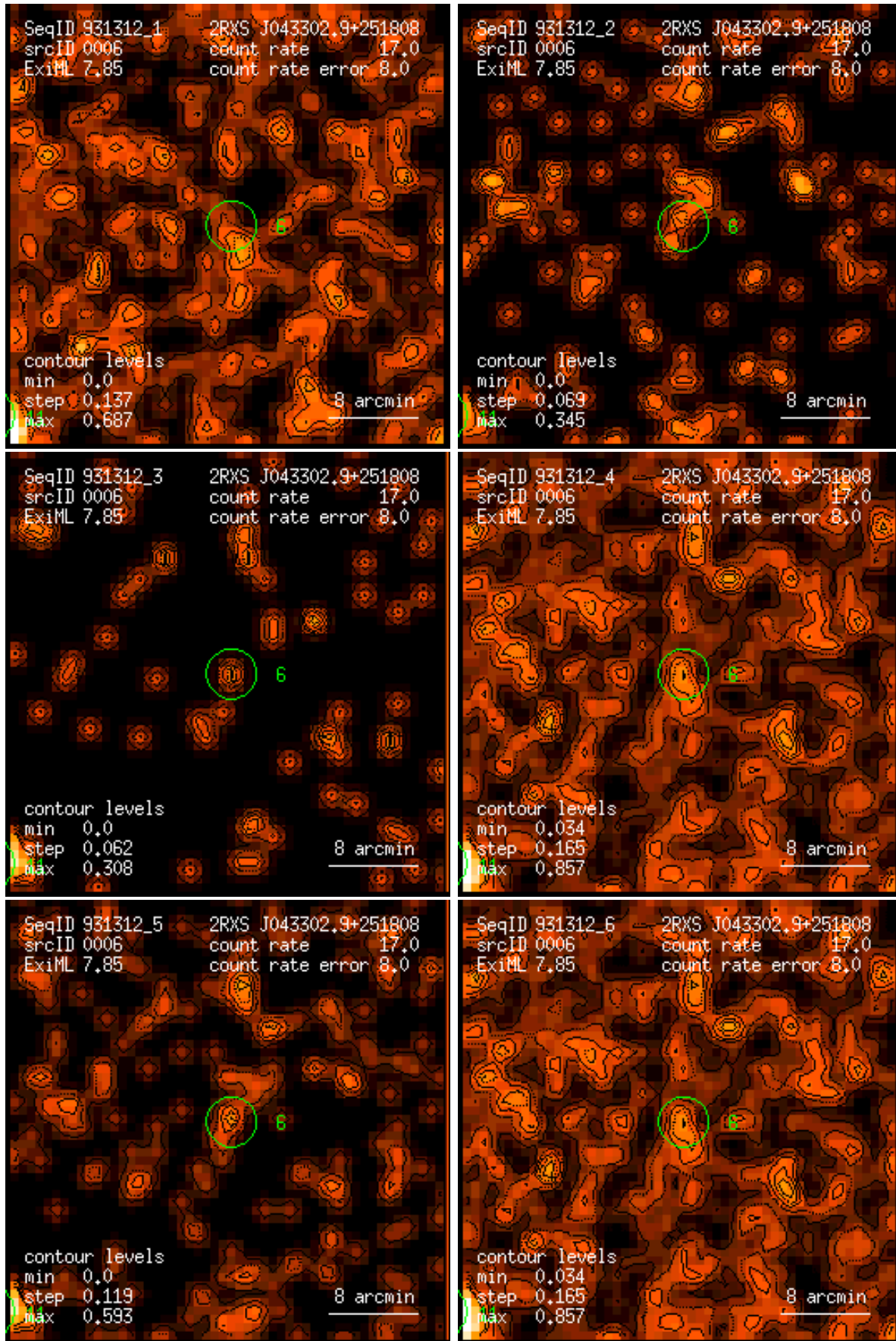
Figure 6: RASS 931312: detection 0006: band rate images, Gaussian filter: (1) PSPC channels 11 – 41, (2) 52 – 90, (3) 91 – 201, (4) 11 – 235, (5) 52 – 201, (6) 11 – 201. Broad band rates in counts/ks. Band rate contour levels in counts/ks/arcmin 2 .
