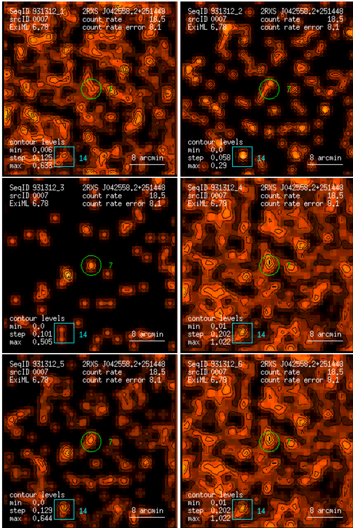
Figure 7: RASS 931312: detection 0007: band rate images, Gaussian filter: (1) PSPC channels 11 – 41, (2) 52 – 90, (3) 91 – 201, (4) 11 – 235, (5) 52 – 201, (6) 11 – 201. Broad band rates in counts/ks. Band rate contour levels in counts/ks/arcmin 2 .
