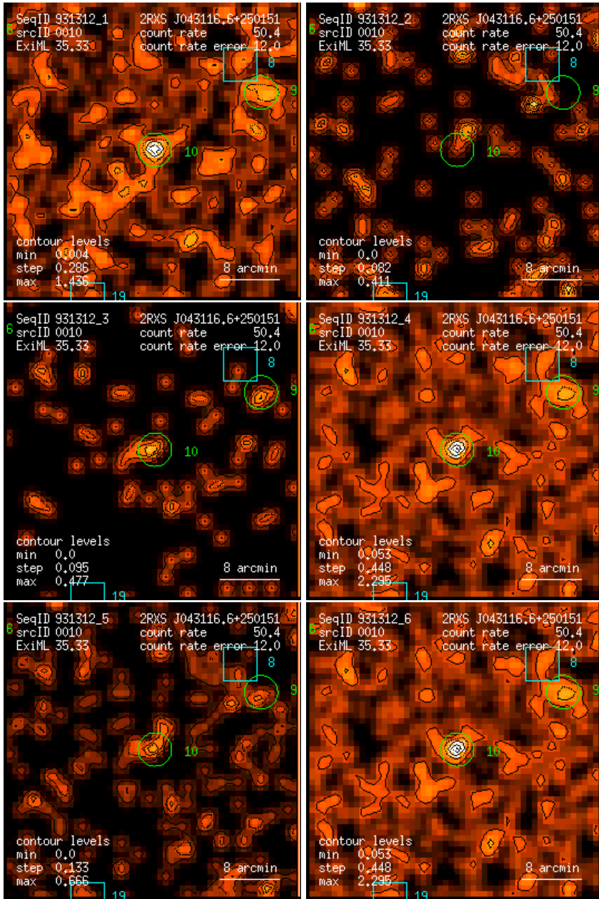
Figure 10: RASS 931312: detection 0010: band rate images, Gaussian filter: (1) PSPC channels 11 – 41, (2) 52 – 90, (3) 91 – 201, (4) 11 – 235, (5) 52 – 201, (6) 11 – 201. Broad band rates in counts/ks. Band rate contour levels in counts/ks/arcmin 2 .
