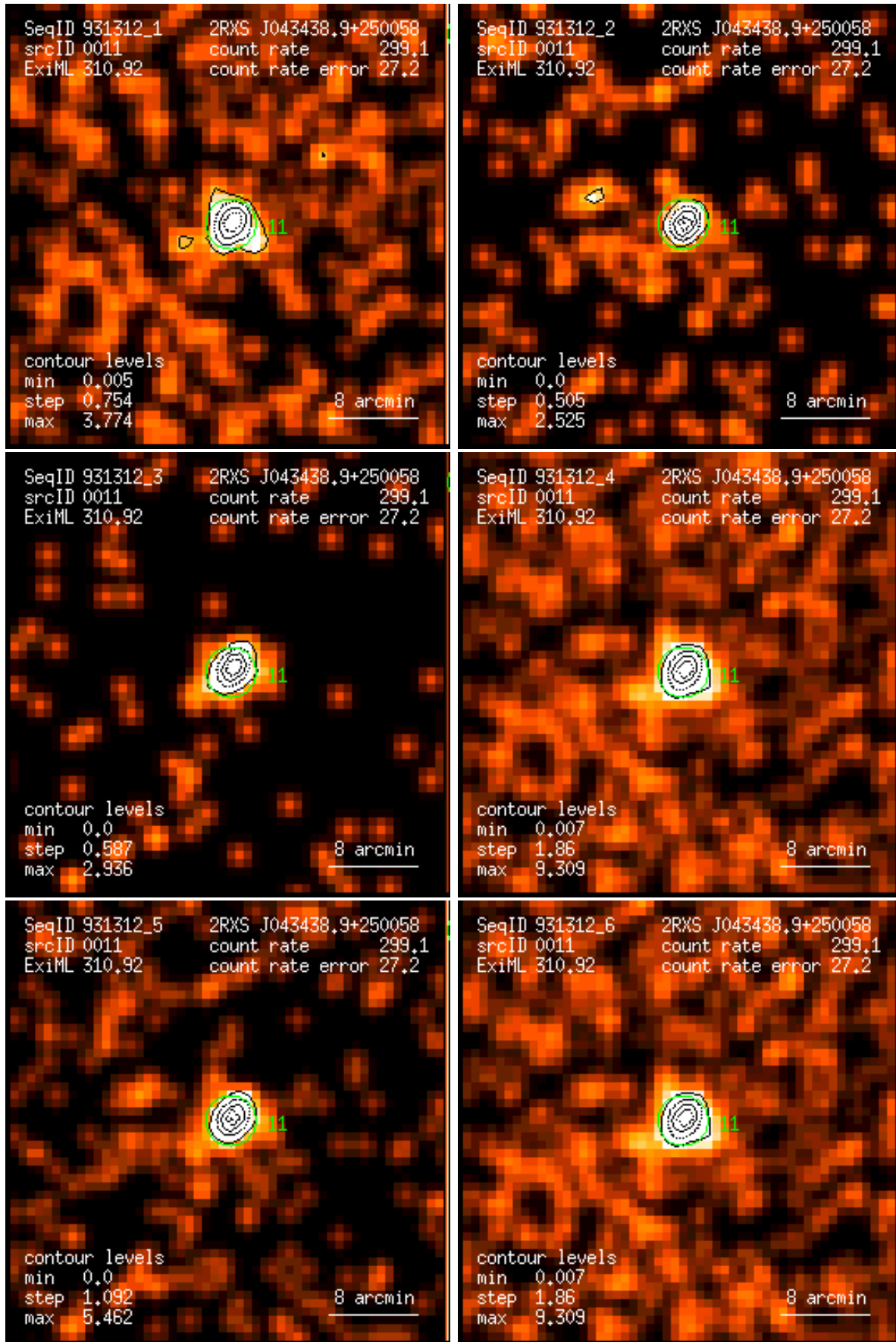
Figure 11: RASS 931312: detection 0011: band rate images, Gaussian filter: (1) PSPC channels 11 – 41, (2) 52 – 90, (3) 91 – 201, (4) 11 – 235, (5) 52 – 201, (6) 11 – 201. Broad band rates in counts/ks. Band rate contour levels in counts/ks/arcmin 2 .
