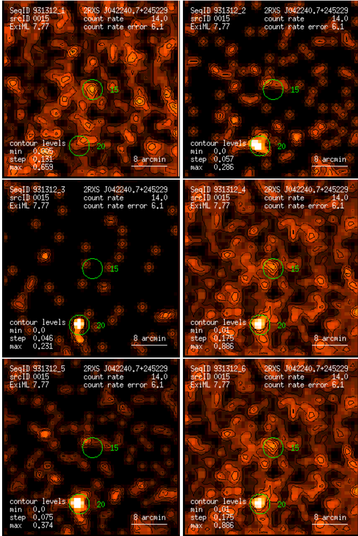
Figure 15: RASS 931312: detection 0015: band rate images, Gaussian filter: (1) PSPC channels 11 – 41, (2) 52 – 90, (3) 91 – 201, (4) 11 – 235, (5) 52 – 201, (6) 11 – 201. Broad band rates in counts/ks. Band rate contour levels in counts/ks/arcmin 2 .
