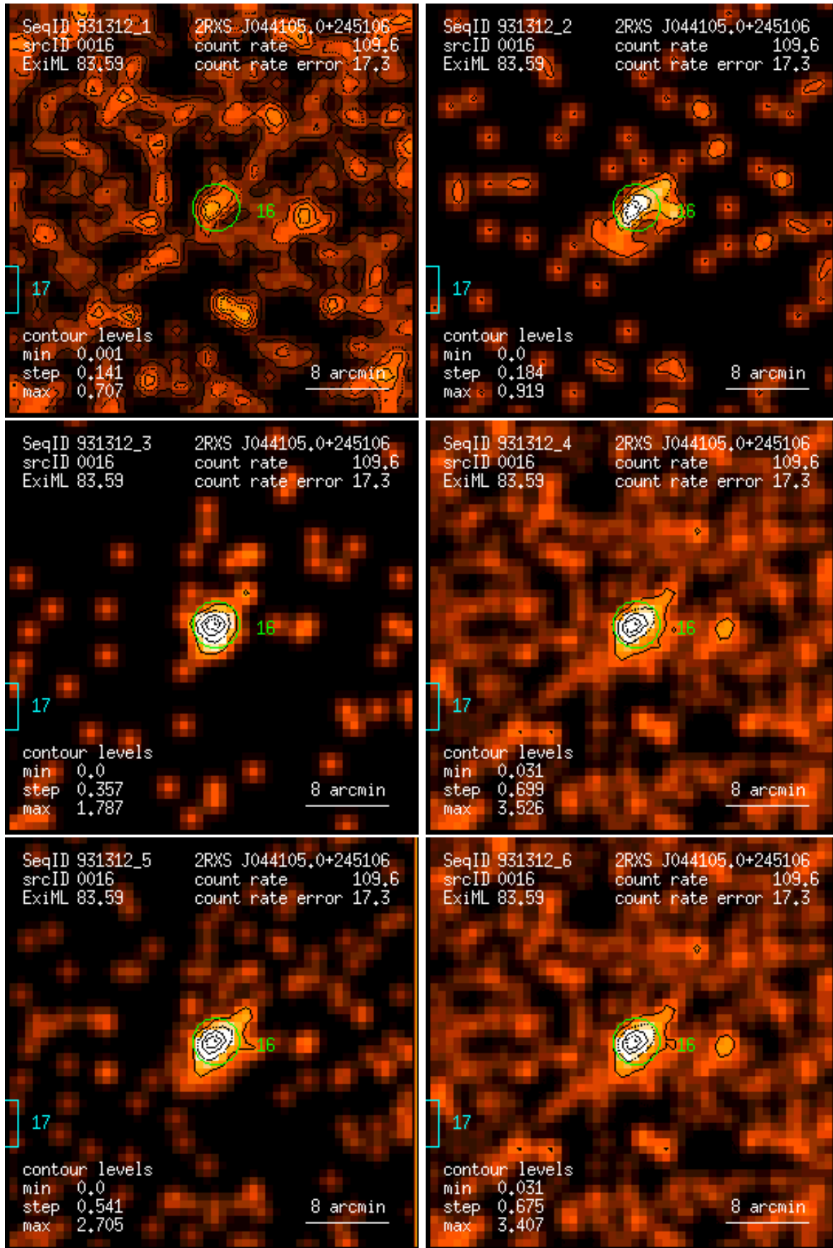
Figure 16: RASS 931312: detection 0016: band rate images, Gaussian filter: (1) PSPC channels 11 – 41, (2) 52 – 90, (3) 91 – 201, (4) 11 – 235, (5) 52 – 201, (6) 11 – 201. Broad band rates in counts/ks. Band rate contour levels in counts/ks/arcmin 2 .
