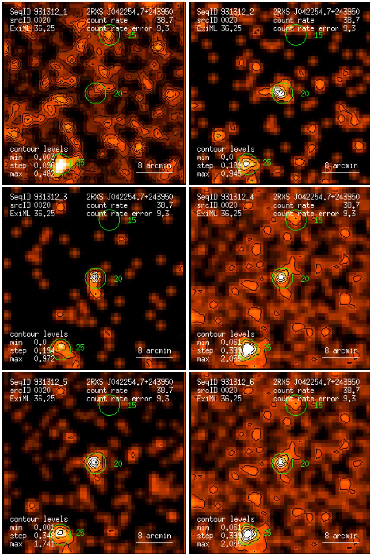
Figure 20: RASS 931312: detection 0020: band rate images, Gaussian filter: (1) PSPC channels 11 – 41, (2) 52 – 90, (3) 91 – 201, (4) 11 – 235, (5) 52 – 201, (6) 11 – 201. Broad band rates in counts/ks. Band rate contour levels in counts/ks/arcmin 2 .
