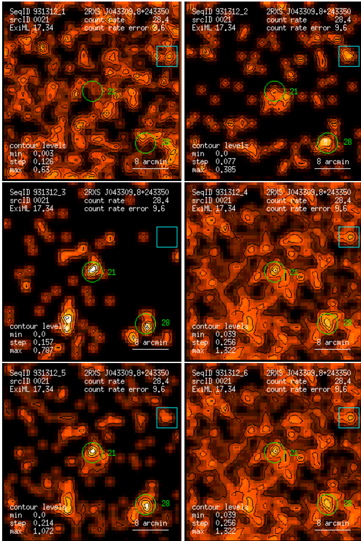
Figure 21: RASS 931312: detection 0021: band rate images, Gaussian filter: (1) PSPC channels 11 – 41, (2) 52 – 90, (3) 91 – 201, (4) 11 – 235, (5) 52 – 201, (6) 11 – 201. Broad band rates in counts/ks. Band rate contour levels in counts/ks/arcmin 2 .
