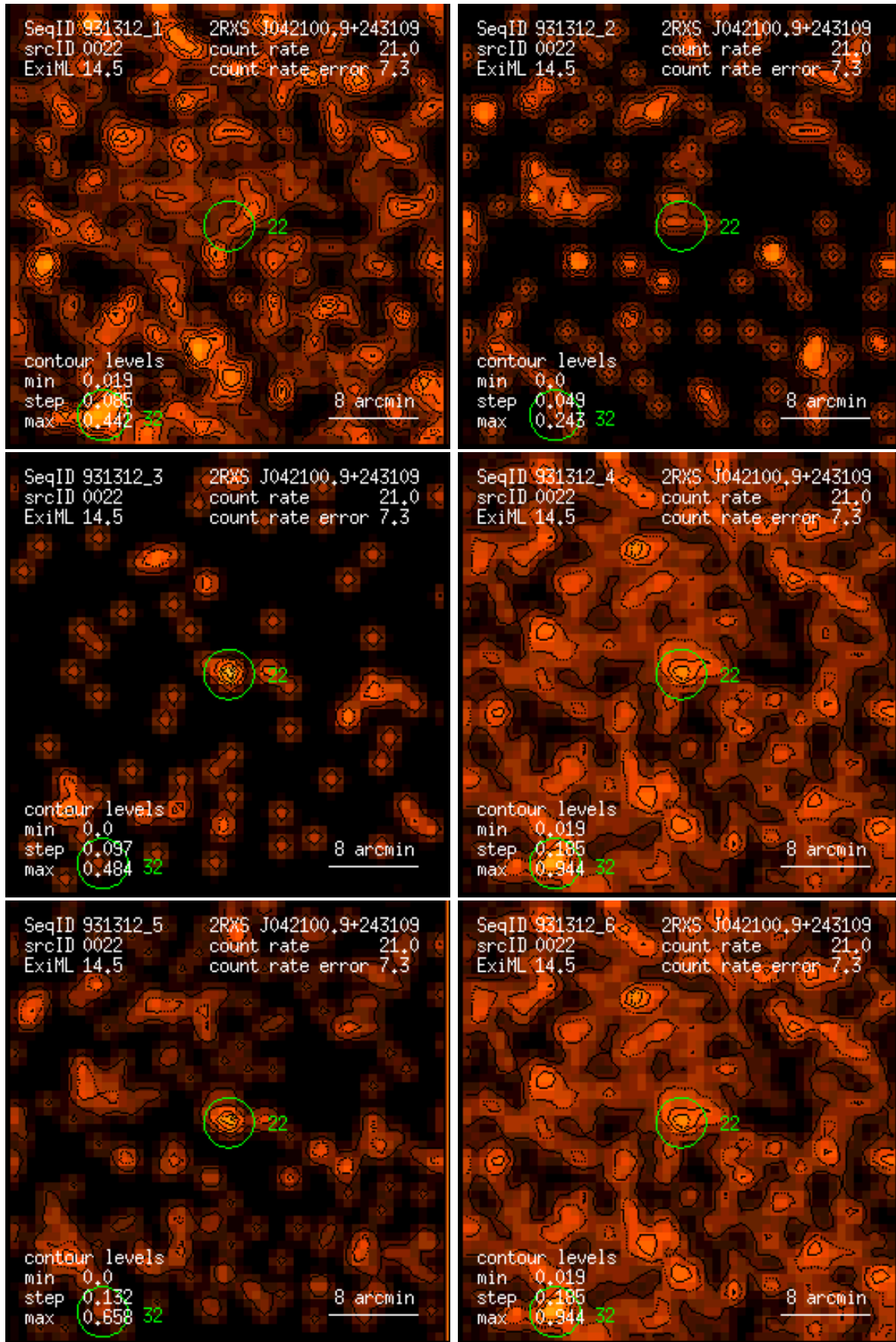
Figure 22: RASS 931312: detection 0022: band rate images, Gaussian filter: (1) PSPC channels 11 – 41, (2) 52 – 90, (3) 91 – 201, (4) 11 – 235, (5) 52 – 201, (6) 11 – 201. Broad band rates in counts/ks. Band rate contour levels in counts/ks/arcmin 2 .
