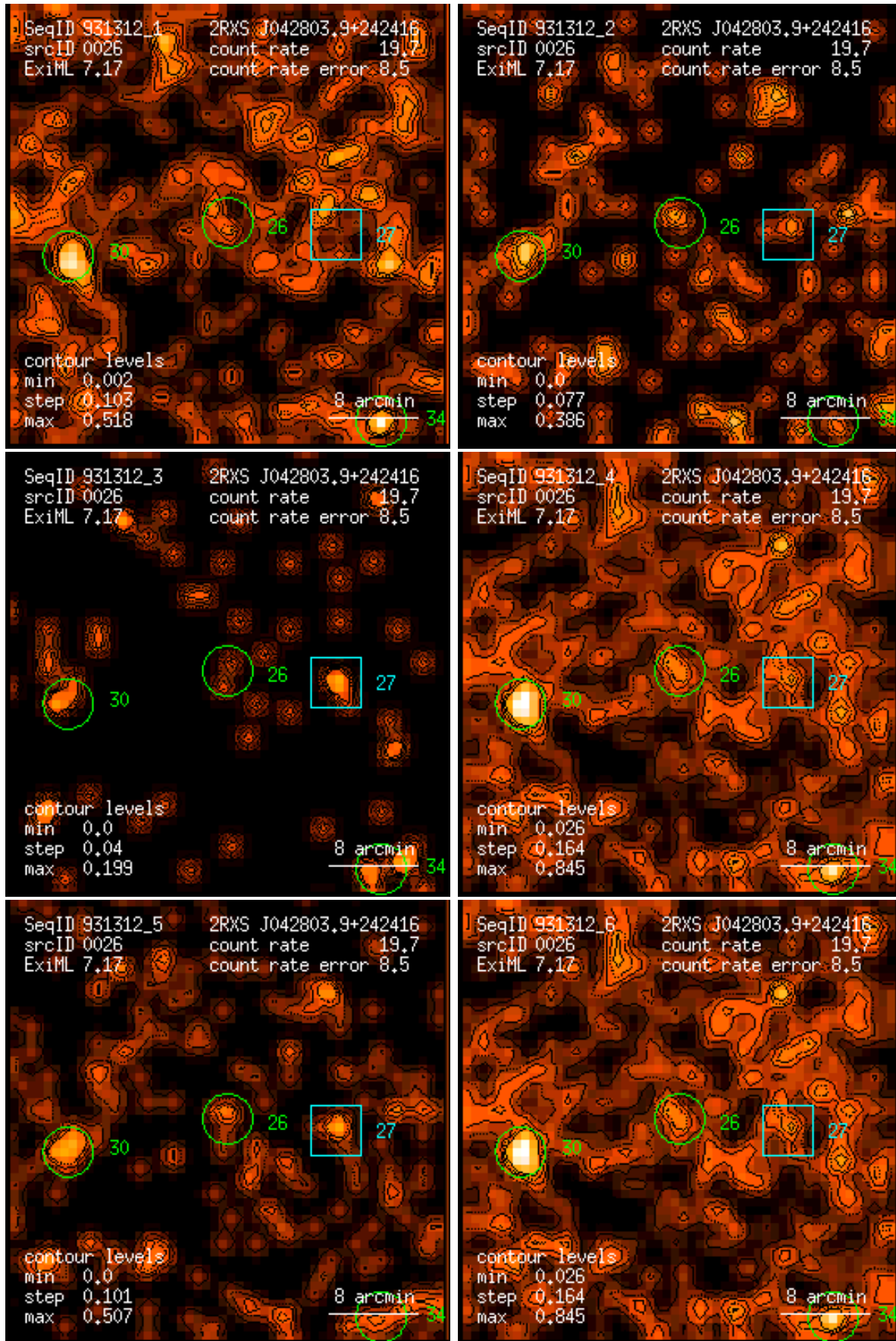
Figure 26: RASS 931312: detection 0026: band rate images, Gaussian filter: (1) PSPC channels 11 – 41, (2) 52 – 90, (3) 91 – 201, (4) 11 – 235, (5) 52 – 201, (6) 11 – 201. Broad band rates in counts/ks. Band rate contour levels in counts/ks/arcmin 2 .
