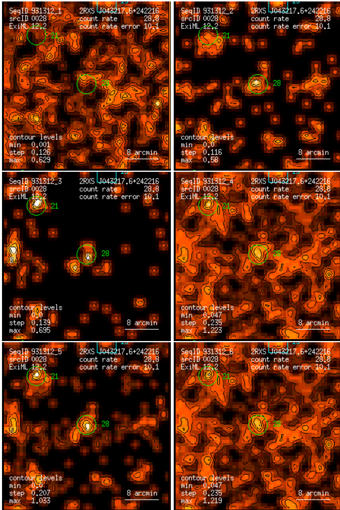
Figure 28: RASS 931312: detection 0028: band rate images, Gaussian filter: (1) PSPC channels 11 – 41, (2) 52 – 90, (3) 91 – 201, (4) 11 – 235, (5) 52 – 201, (6) 11 – 201. Broad band rates in counts/ks. Band rate contour levels in counts/ks/arcmin 2 .
