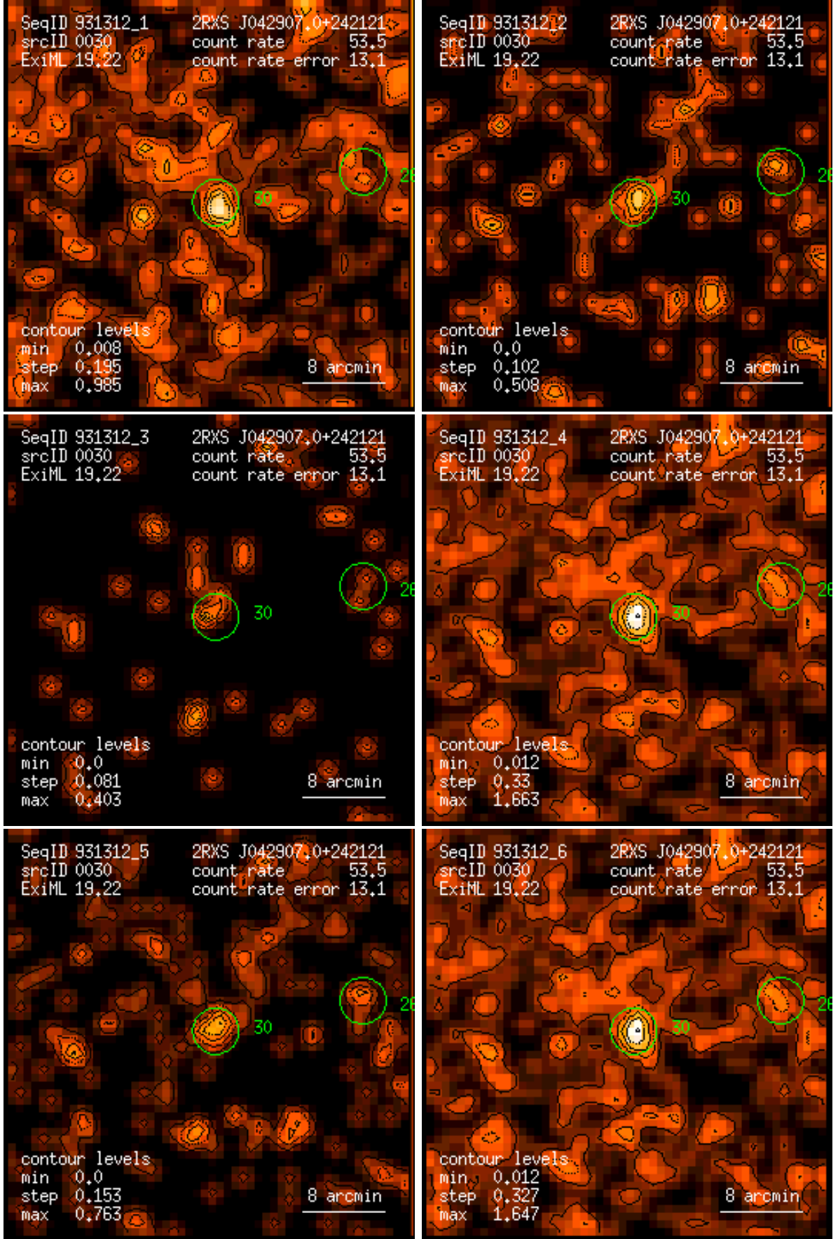
Figure 30: RASS 931312: detection 0030: band rate images, Gaussian filter: (1) PSPC channels 11 – 41, (2) 52 – 90, (3) 91 – 201, (4) 11 – 235, (5) 52 – 201, (6) 11 – 201. Broad band rates in counts/ks. Band rate contour levels in counts/ks/arcmin 2 .
