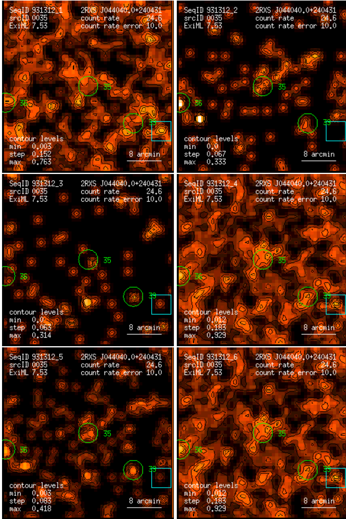
Figure 35: RASS 931312: detection 0035: band rate images, Gaussian filter: (1) PSPC channels 11 – 41, (2) 52 – 90, (3) 91 – 201, (4) 11 – 235, (5) 52 – 201, (6) 11 – 201. Broad band rates in counts/ks. Band rate contour levels in counts/ks/arcmin 2 .
