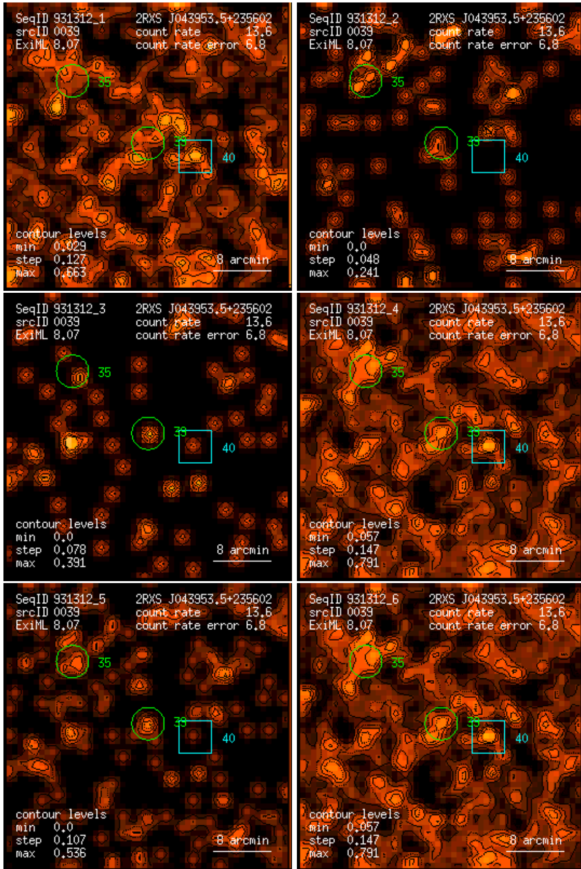
Figure 39: RASS 931312: detection 0039: band rate images, Gaussian filter: (1) PSPC channels 11 – 41, (2) 52 – 90, (3) 91 – 201, (4) 11 – 235, (5) 52 – 201, (6) 11 – 201. Broad band rates in counts/ks. Band rate contour levels in counts/ks/arcmin 2 .
