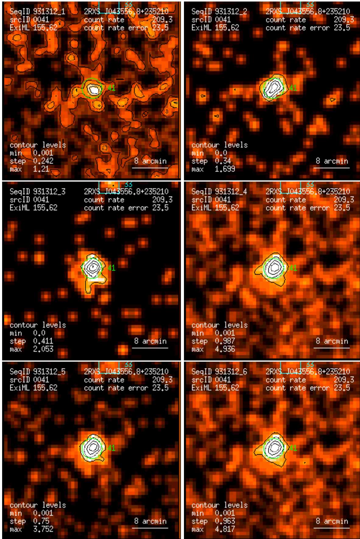
Figure 41: RASS 931312: detection 0041: band rate images, Gaussian filter: (1) PSPC channels 11 – 41, (2) 52 – 90, (3) 91 – 201, (4) 11 – 235, (5) 52 – 201, (6) 11 – 201. Broad band rates in counts/ks. Band rate contour levels in counts/ks/arcmin 2 .
