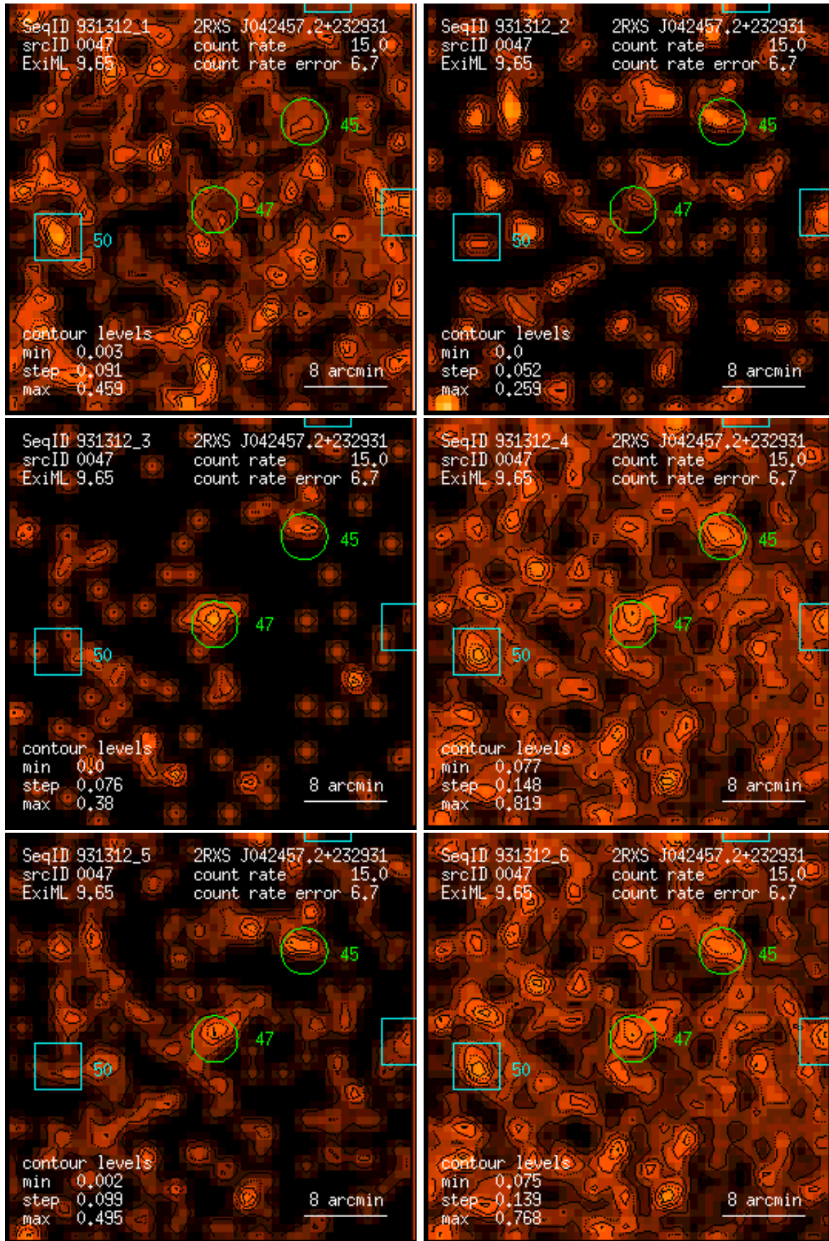
Figure 47: RASS 931312: detection 0047: band rate images, Gaussian filter: (1) PSPC channels 11 – 41, (2) 52 – 90, (3) 91 – 201, (4) 11 – 235, (5) 52 – 201, (6) 11 – 201. Broad band rates in counts/ks. Band rate contour levels in counts/ks/arcmin 2 .
