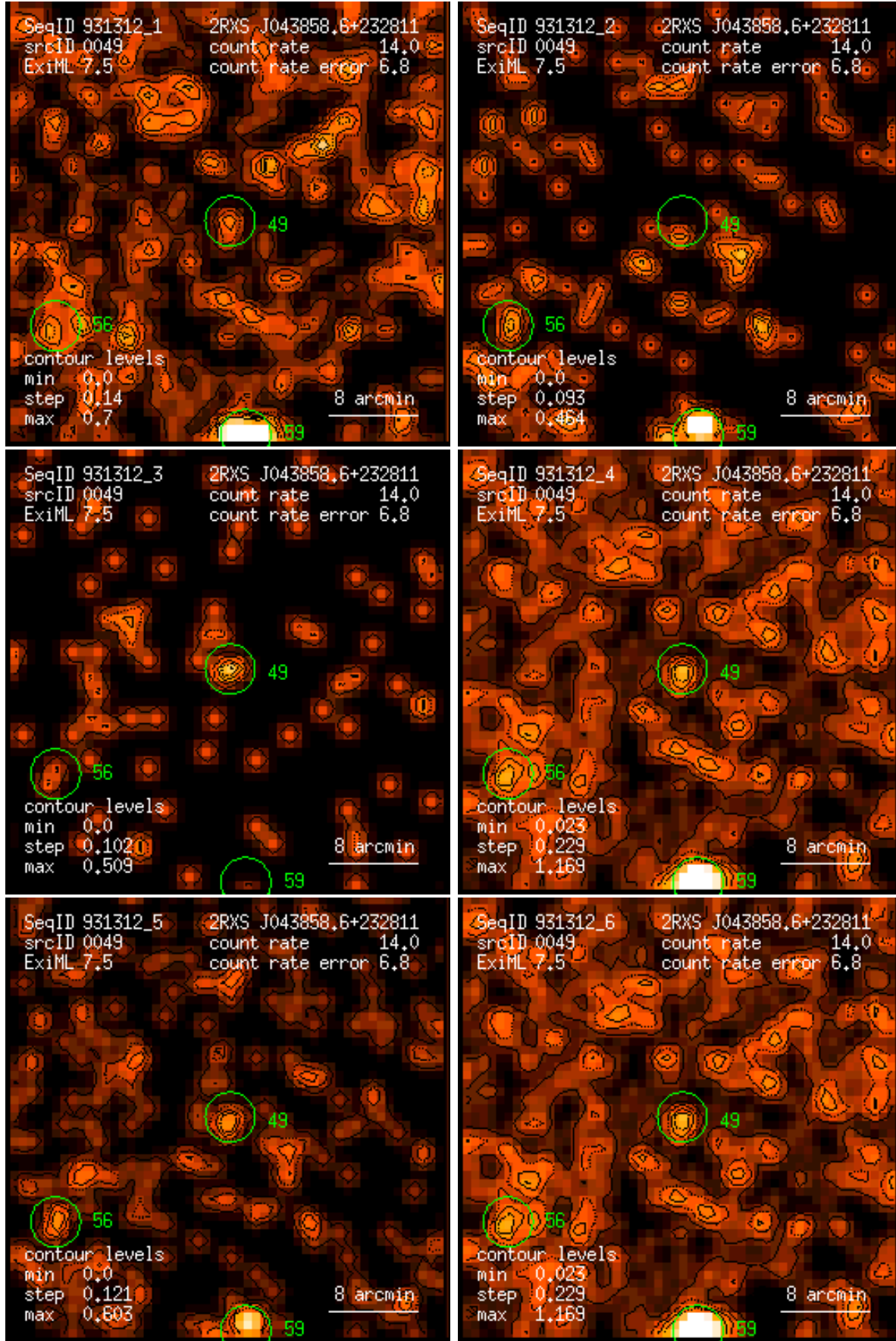
Figure 49: RASS 931312: detection 0049: band rate images, Gaussian filter: (1) PSPC channels 11 – 41, (2) 52 – 90, (3) 91 – 201, (4) 11 – 235, (5) 52 – 201, (6) 11 – 201. Broad band rates in counts/ks. Band rate contour levels in counts/ks/arcmin 2 .
