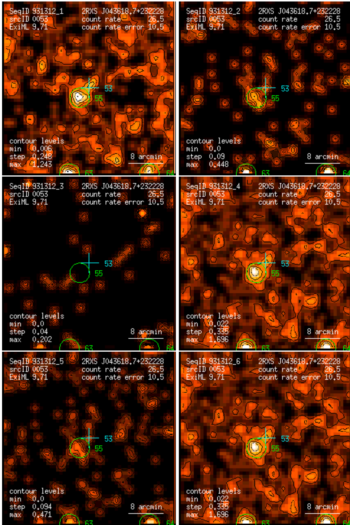
Figure 53: RASS 931312: detection 0053: band rate images, Gaussian filter: (1) PSPC channels 11 – 41, (2) 52 – 90, (3) 91 – 201, (4) 11 – 235, (5) 52 – 201, (6) 11 – 201. Broad band rates in counts/ks. Band rate contour levels in counts/ks/arcmin 2 .
