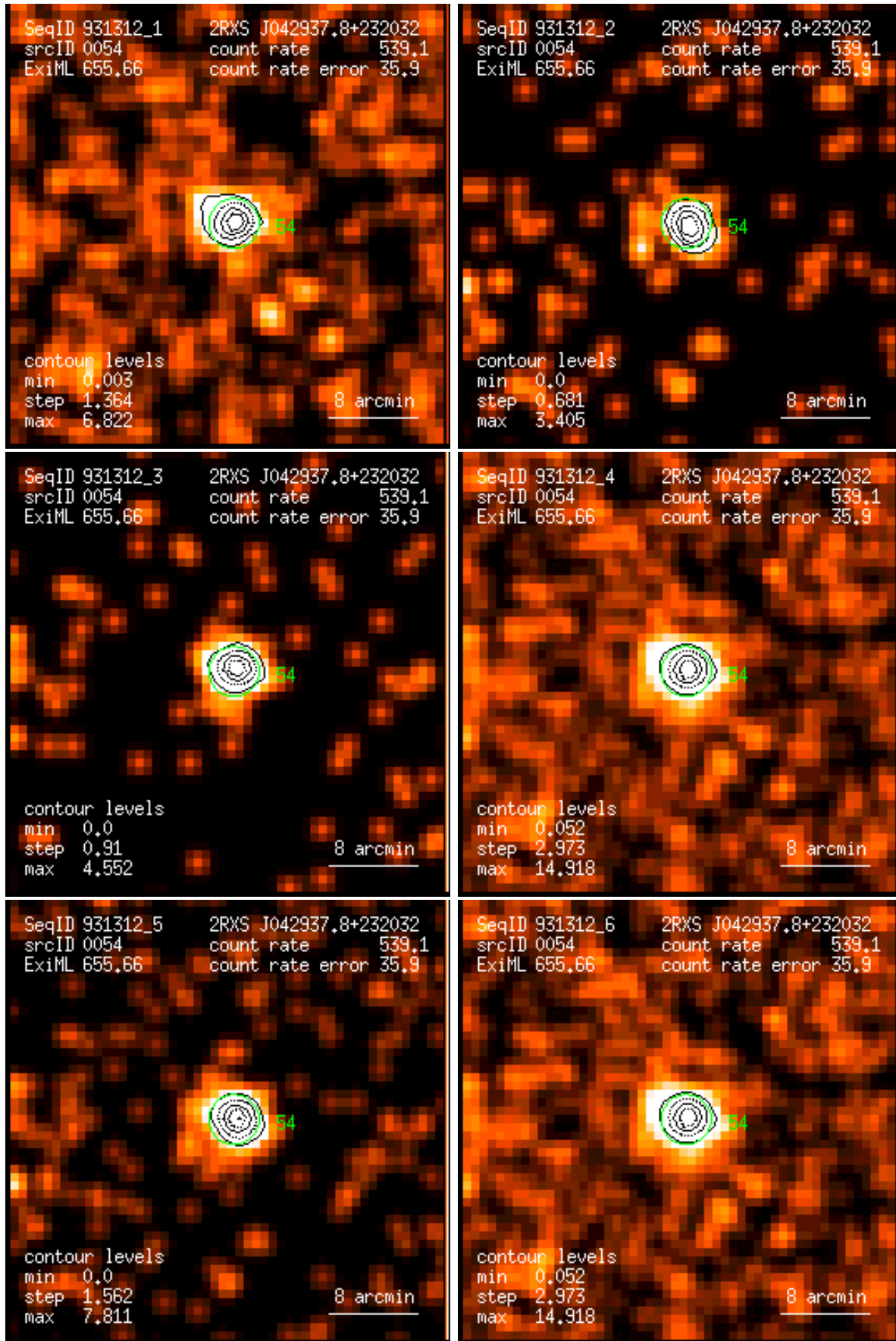
Figure 54: RASS 931312: detection 0054: band rate images, Gaussian filter: (1) PSPC channels 11 – 41, (2) 52 – 90, (3) 91 – 201, (4) 11 – 235, (5) 52 – 201, (6) 11 – 201. Broad band rates in counts/ks. Band rate contour levels in counts/ks/arcmin 2 .
