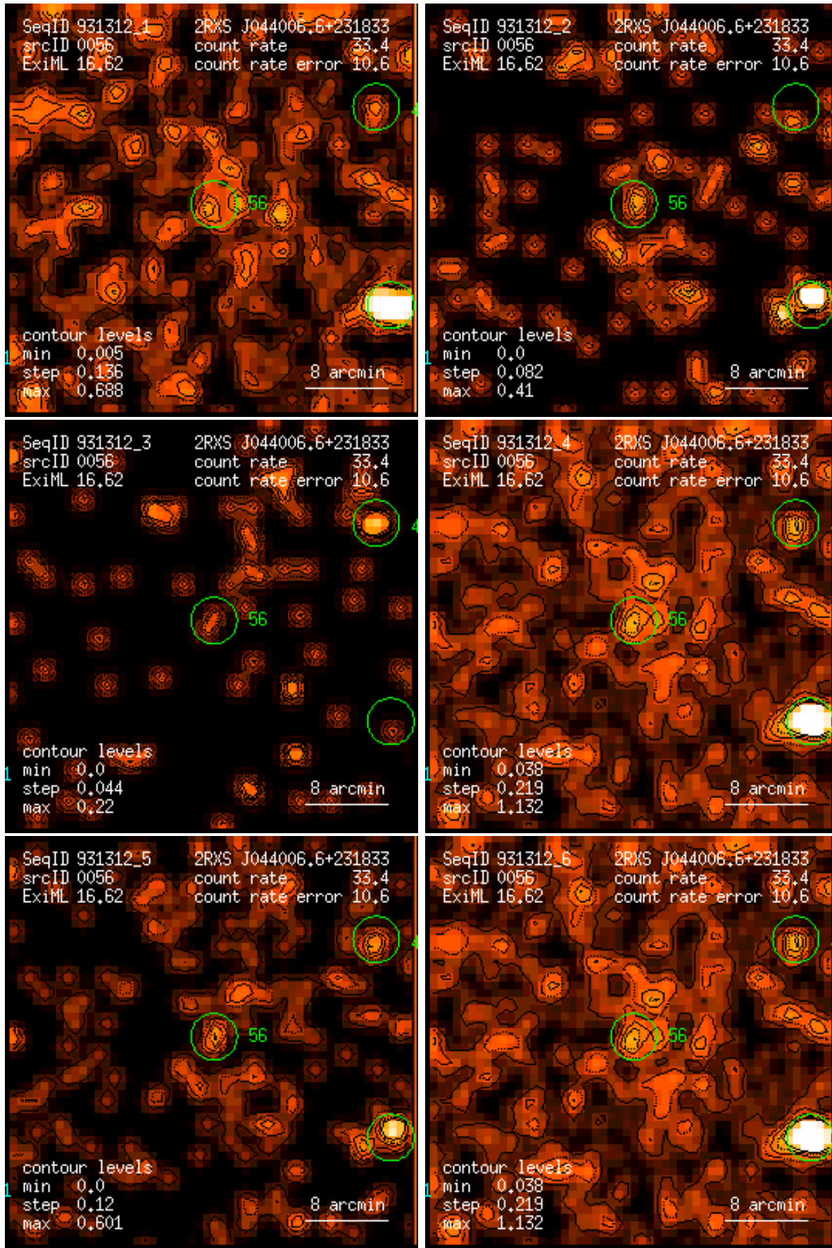
Figure 56: RASS 931312: detection 0056: band rate images, Gaussian filter: (1) PSPC channels 11 – 41, (2) 52 – 90, (3) 91 – 201, (4) 11 – 235, (5) 52 – 201, (6) 11 – 201. Broad band rates in counts/ks. Band rate contour levels in counts/ks/arcmin 2 .
