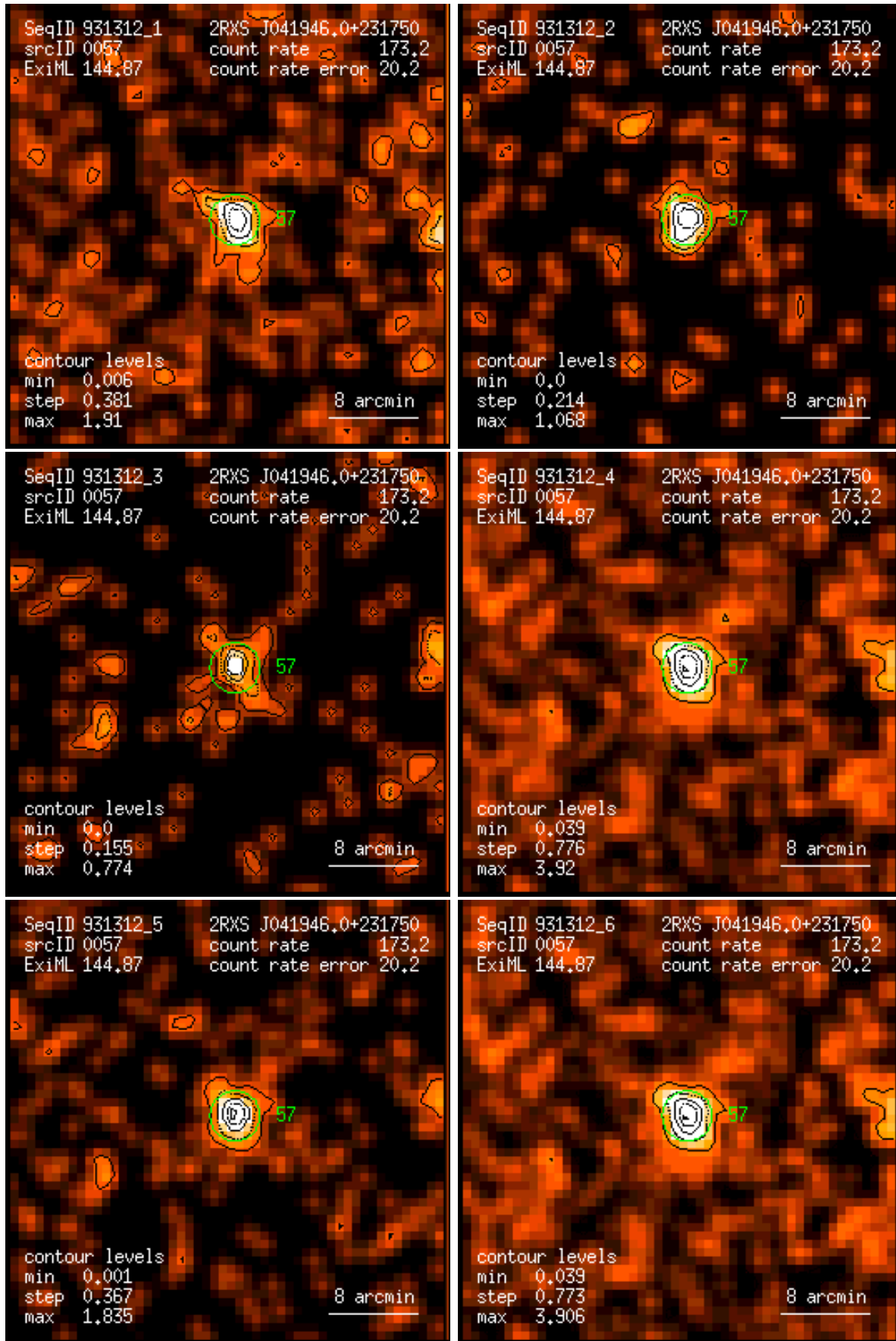
Figure 57: RASS 931312: detection 0057: band rate images, Gaussian filter: (1) PSPC channels 11 – 41, (2) 52 – 90, (3) 91 – 201, (4) 11 – 235, (5) 52 – 201, (6) 11 – 201. Broad band rates in counts/ks. Band rate contour levels in counts/ks/arcmin 2 .
