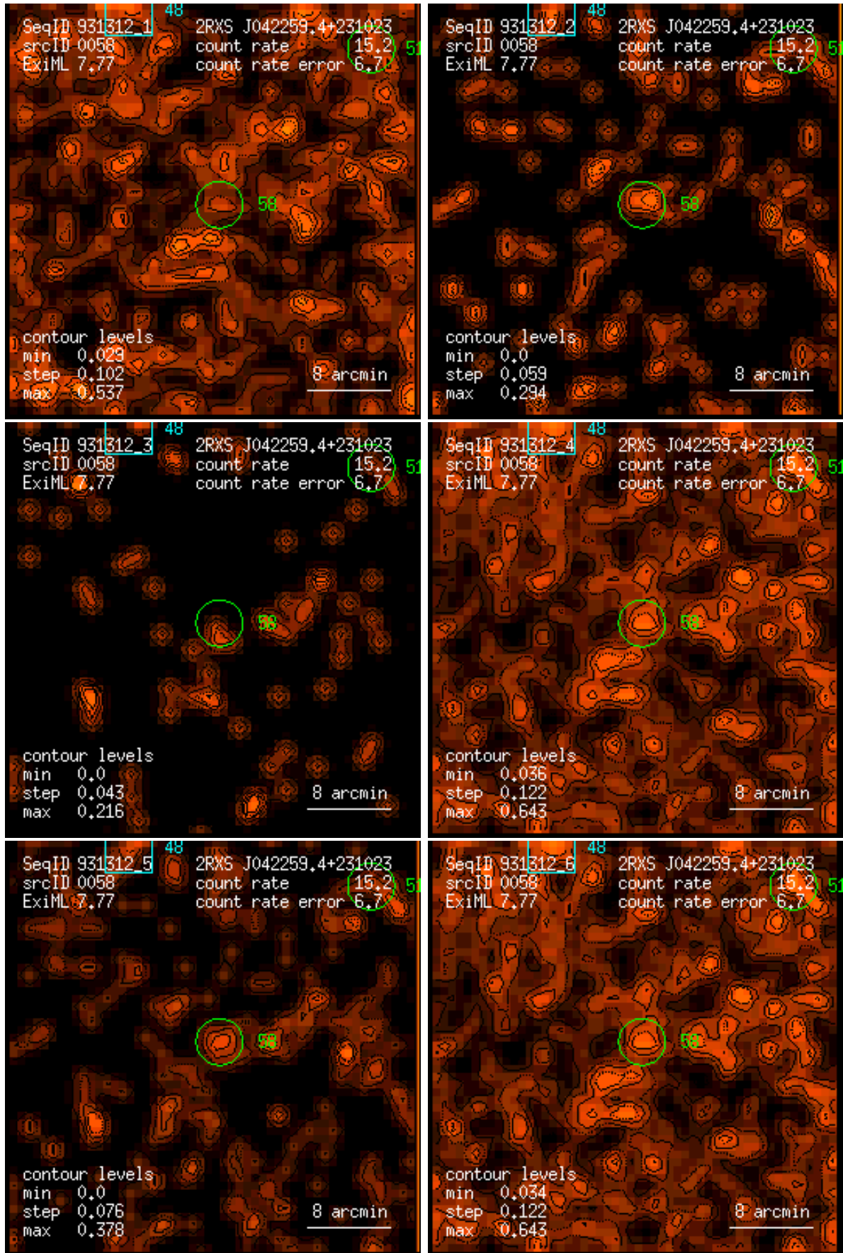
Figure 58: RASS 931312: detection 0058: band rate images, Gaussian filter: (1) PSPC channels 11 – 41, (2) 52 – 90, (3) 91 – 201, (4) 11 – 235, (5) 52 – 201, (6) 11 – 201. Broad band rates in counts/ks. Band rate contour levels in counts/ks/arcmin 2 .
