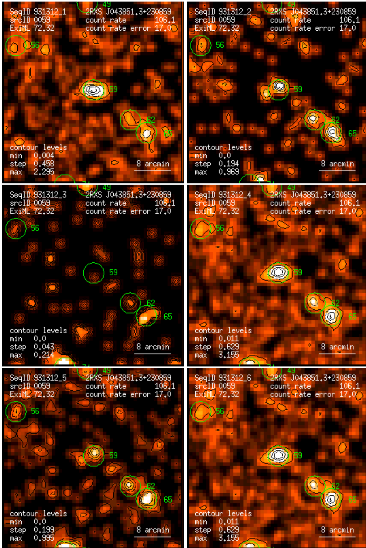
Figure 59: RASS 931312: detection 0059: band rate images, Gaussian filter: (1) PSPC channels 11 – 41, (2) 52 – 90, (3) 91 – 201, (4) 11 – 235, (5) 52 – 201, (6) 11 – 201. Broad band rates in counts/ks. Band rate contour levels in counts/ks/arcmin 2 .
