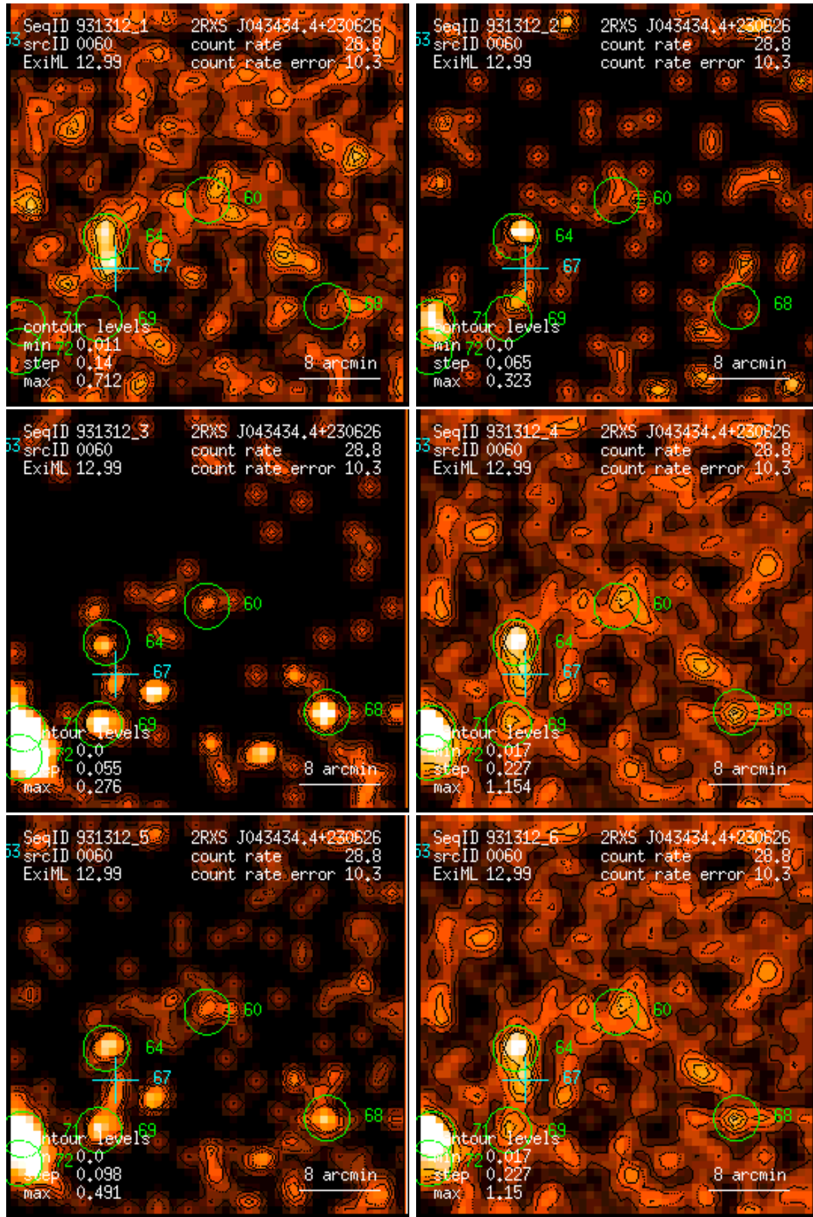
Figure 60: RASS 931312: detection 0060: band rate images, Gaussian filter: (1) PSPC channels 11 – 41, (2) 52 – 90, (3) 91 – 201, (4) 11 – 235, (5) 52 – 201, (6) 11 – 201. Broad band rates in counts/ks. Band rate contour levels in counts/ks/arcmin 2 .
