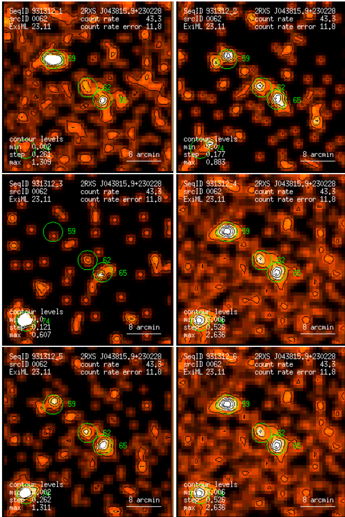
Figure 62: RASS 931312: detection 0062: band rate images, Gaussian filter: (1) PSPC channels 11 – 41, (2) 52 – 90, (3) 91 – 201, (4) 11 – 235, (5) 52 – 201, (6) 11 – 201. Broad band rates in counts/ks. Band rate contour levels in counts/ks/arcmin 2 .
