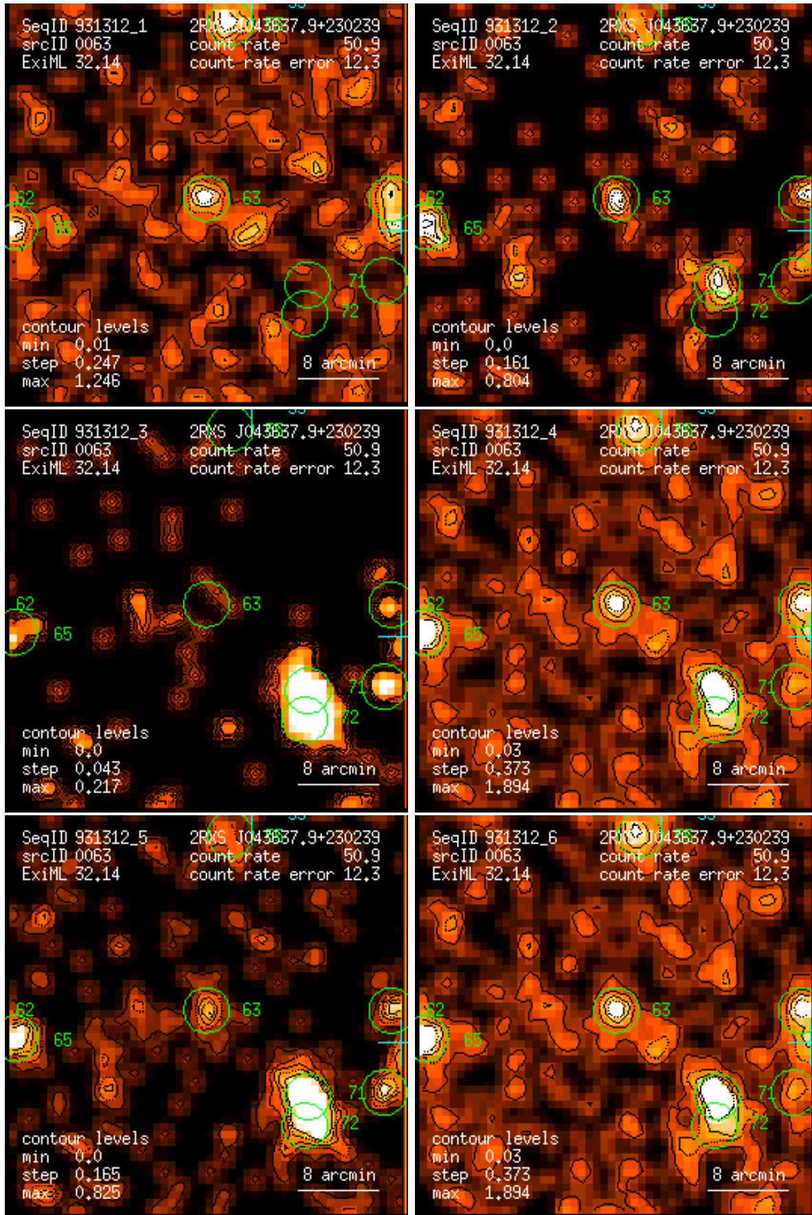
Figure 63: RASS 931312: detection 0063: band rate images, Gaussian filter: (1) PSPC channels 11 – 41, (2) 52 – 90, (3) 91 – 201, (4) 11 – 235, (5) 52 – 201, (6) 11 – 201. Broad band rates in counts/ks. Band rate contour levels in counts/ks/arcmin 2 .
