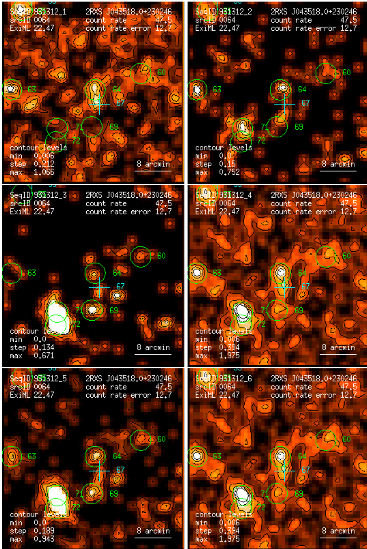
Figure 64: RASS 931312: detection 0064: band rate images, Gaussian filter: (1) PSPC channels 11 – 41, (2) 52 – 90, (3) 91 – 201, (4) 11 – 235, (5) 52 – 201, (6) 11 – 201. Broad band rates in counts/ks. Band rate contour levels in counts/ks/arcmin 2 .
