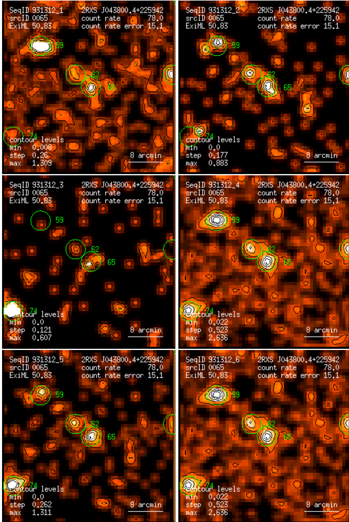
Figure 65: RASS 931312: detection 0065: band rate images, Gaussian filter: (1) PSPC channels 11 – 41, (2) 52 – 90, (3) 91 – 201, (4) 11 – 235, (5) 52 – 201, (6) 11 – 201. Broad band rates in counts/ks. Band rate contour levels in counts/ks/arcmin 2 .
