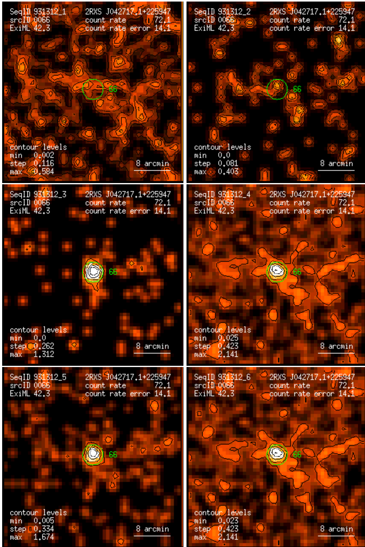
Figure 66: RASS 931312: detection 0066: band rate images, Gaussian filter: (1) PSPC channels 11 – 41, (2) 52 – 90, (3) 91 – 201, (4) 11 – 235, (5) 52 – 201, (6) 11 – 201. Broad band rates in counts/ks. Band rate contour levels in counts/ks/arcmin 2 .
