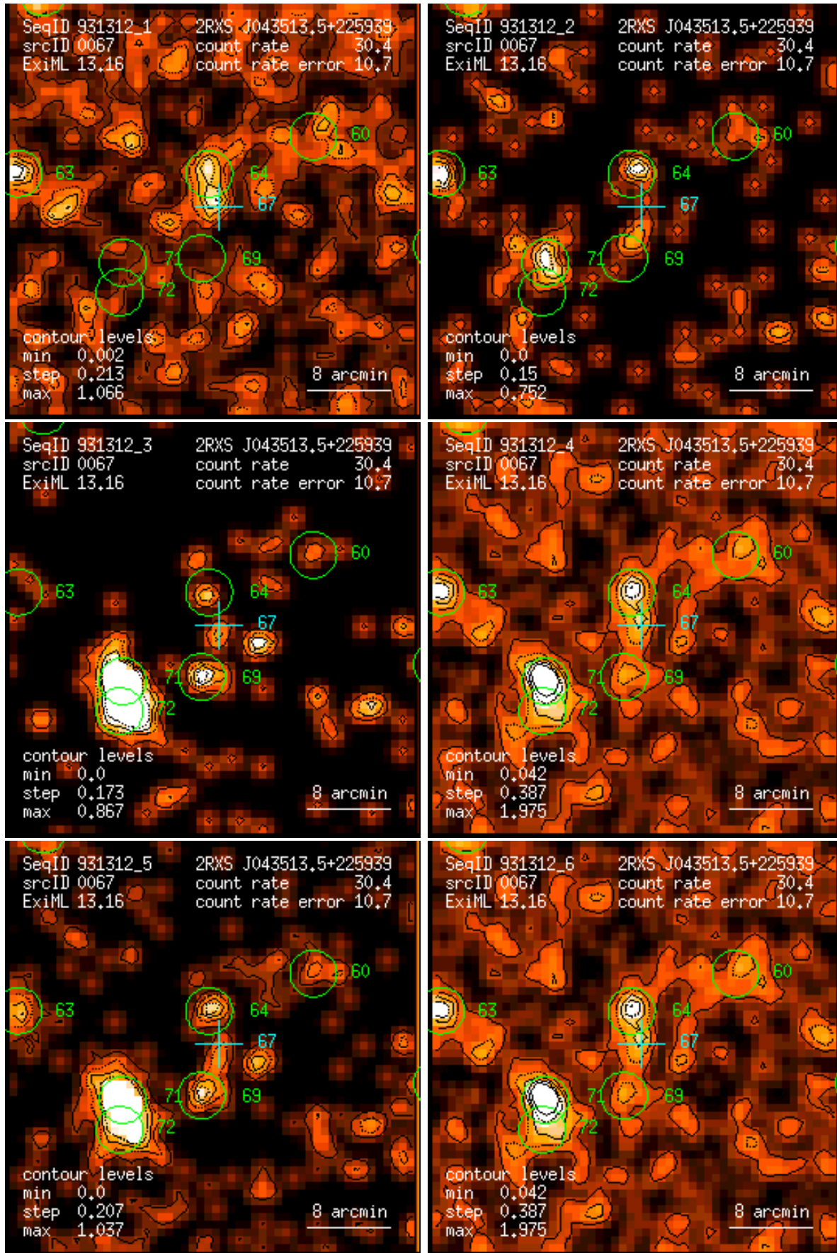
Figure 67: RASS 931312: detection 0067: band rate images, Gaussian filter: (1) PSPC channels 11 – 41, (2) 52 – 90, (3) 91 – 201, (4) 11 – 235, (5) 52 – 201, (6) 11 – 201. Broad band rates in counts/ks. Band rate contour levels in counts/ks/arcmin 2 .
