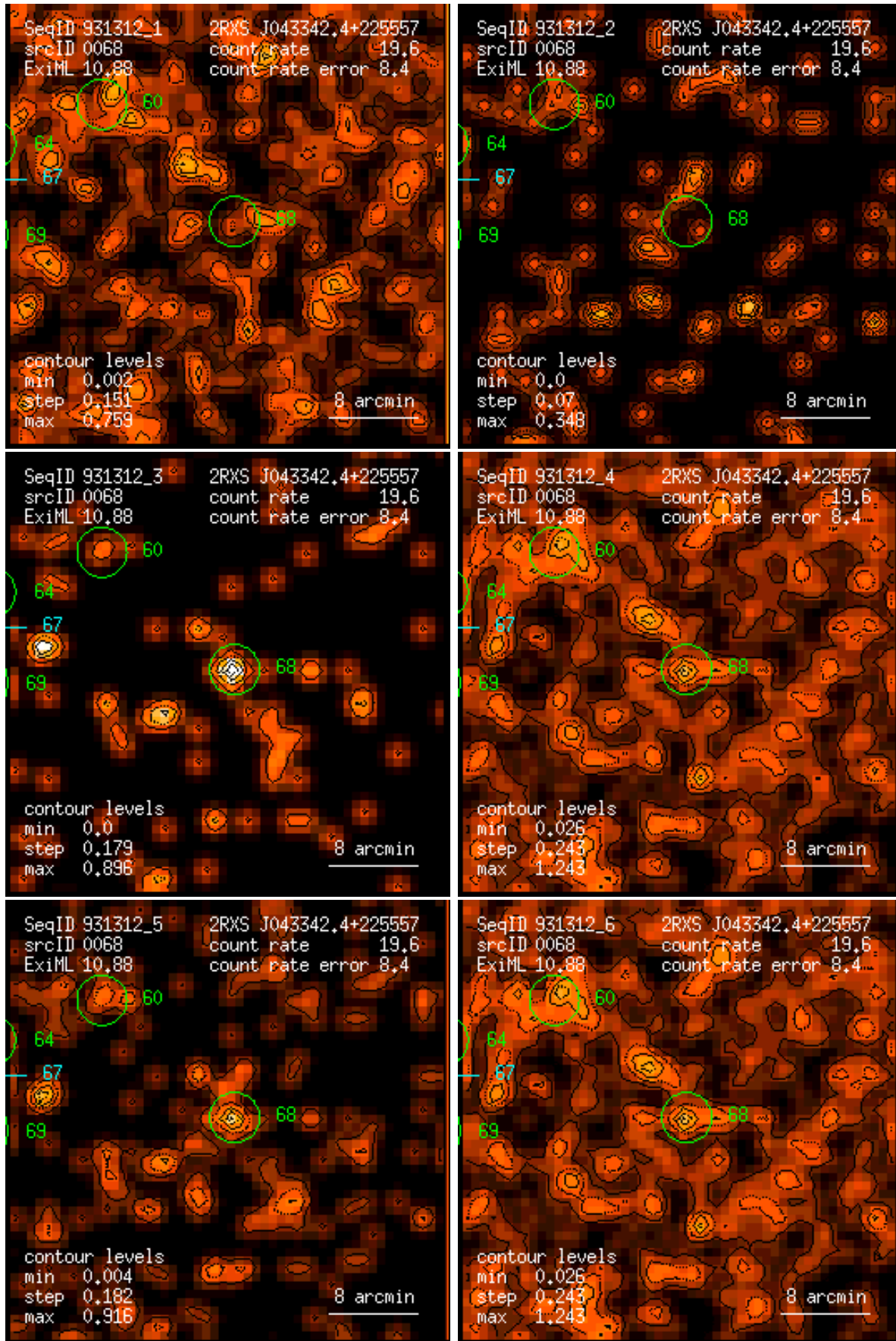
Figure 68: RASS 931312: detection 0068: band rate images, Gaussian filter: (1) PSPC channels 11 – 41, (2) 52 – 90, (3) 91 – 201, (4) 11 – 235, (5) 52 – 201, (6) 11 – 201. Broad band rates in counts/ks. Band rate contour levels in counts/ks/arcmin 2 .
