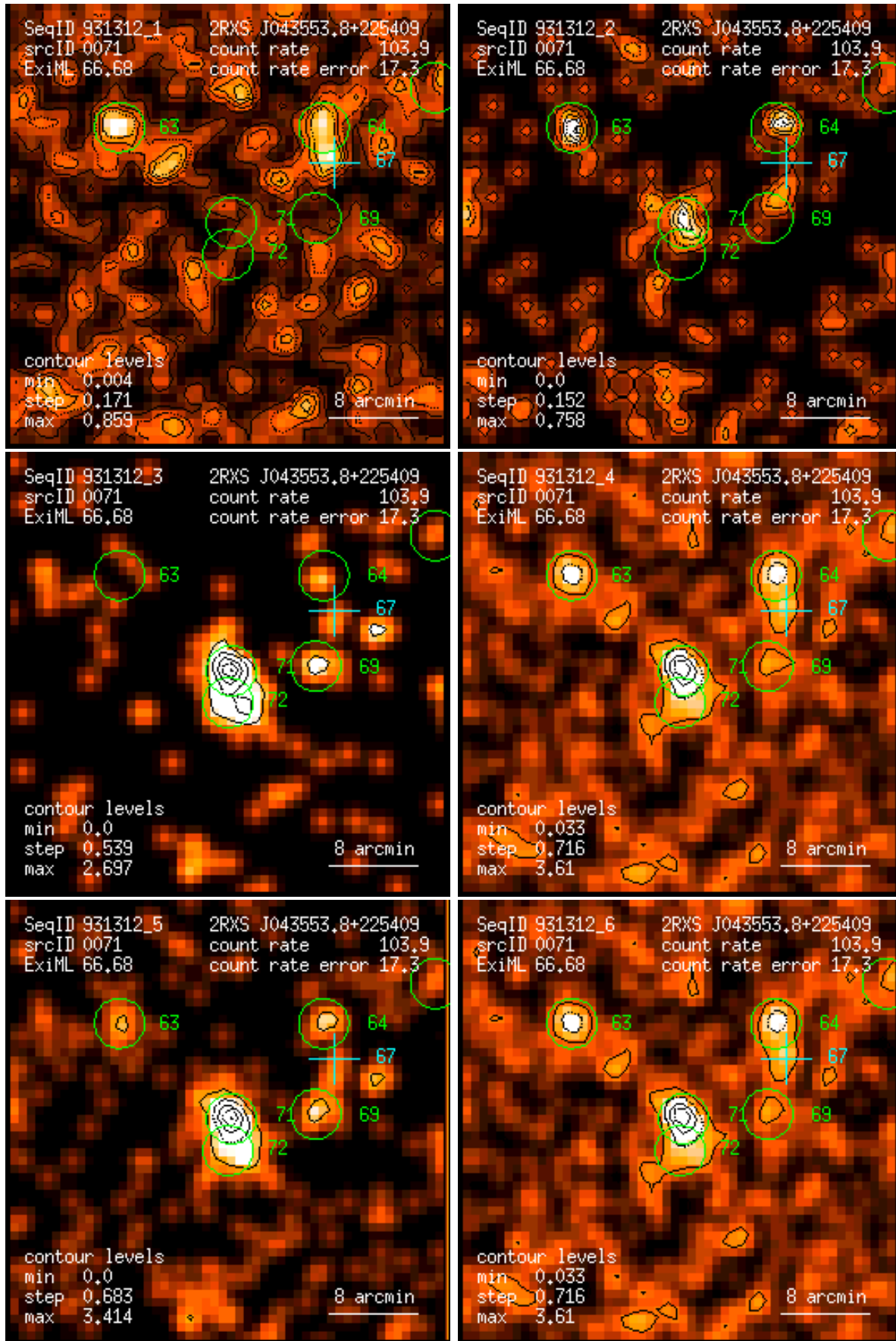
Figure 71: RASS 931312: detection 0071: band rate images, Gaussian filter: (1) PSPC channels 11 – 41, (2) 52 – 90, (3) 91 – 201, (4) 11 – 235, (5) 52 – 201, (6) 11 – 201. Broad band rates in counts/ks. Band rate contour levels in counts/ks/arcmin 2 .
