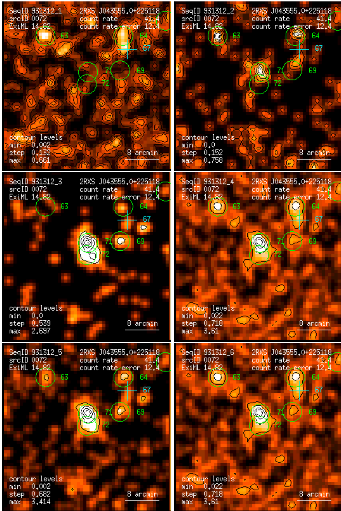
Figure 72: RASS 931312: detection 0072: band rate images, Gaussian filter: (1) PSPC channels 11 – 41, (2) 52 – 90, (3) 91 – 201, (4) 11 – 235, (5) 52 – 201, (6) 11 – 201. Broad band rates in counts/ks. Band rate contour levels in counts/ks/arcmin 2 .
