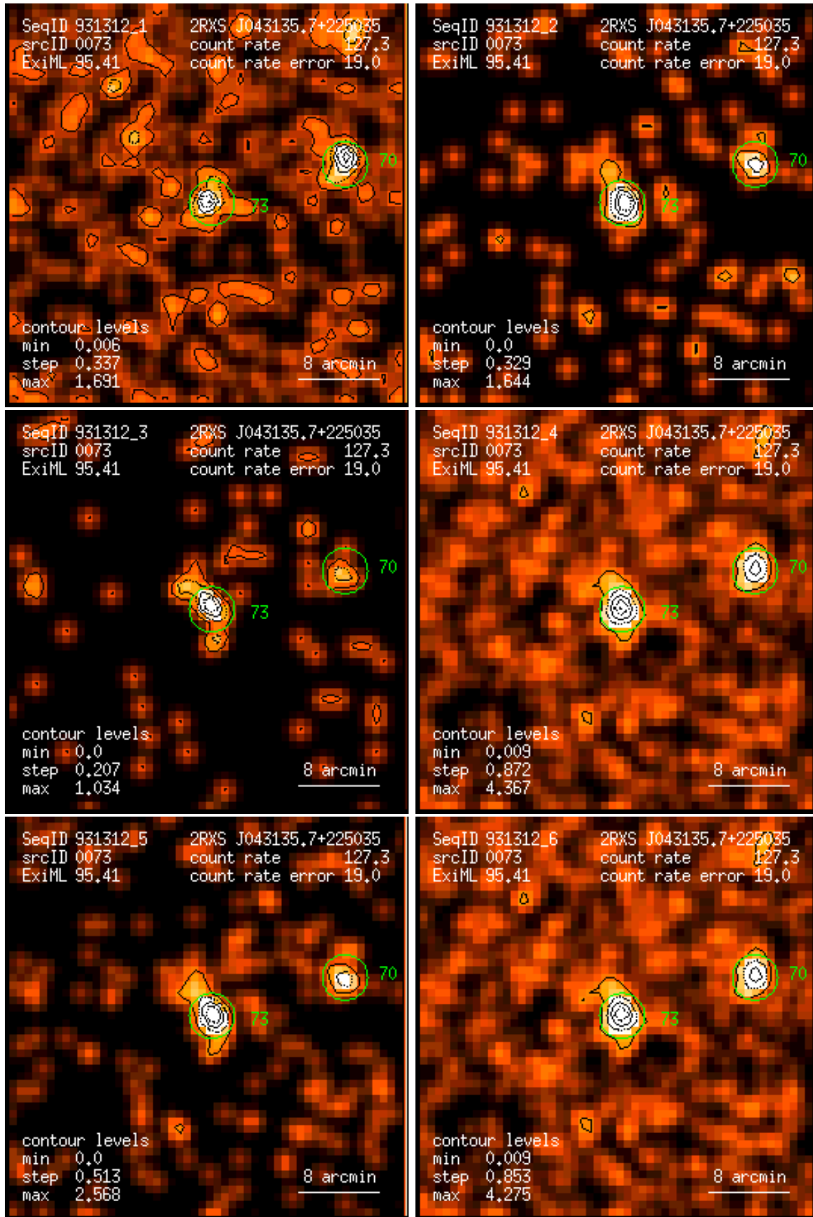
Figure 73: RASS 931312: detection 0073: band rate images, Gaussian filter: (1) PSPC channels 11 – 41, (2) 52 – 90, (3) 91 – 201, (4) 11 – 235, (5) 52 – 201, (6) 11 – 201. Broad band rates in counts/ks. Band rate contour levels in counts/ks/arcmin 2 .
