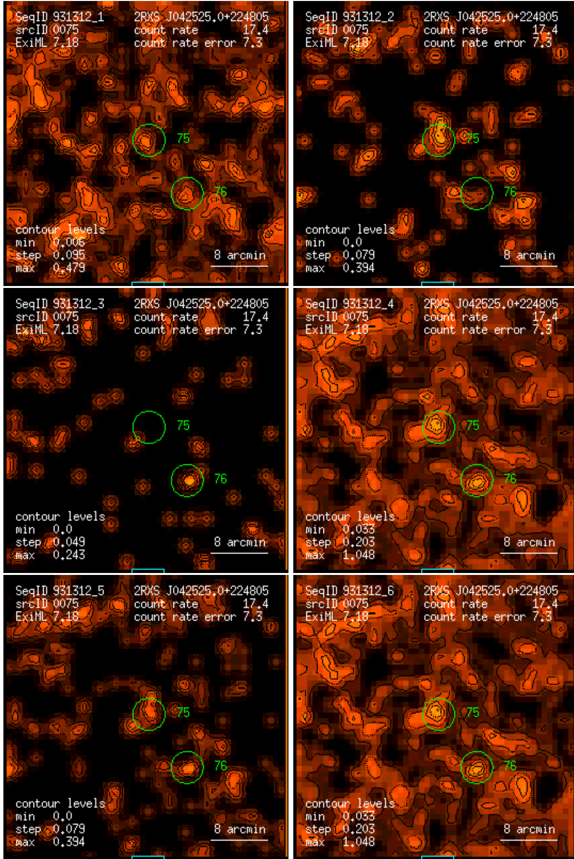
Figure 75: RASS 931312: detection 0075: band rate images, Gaussian filter: (1) PSPC channels 11 – 41, (2) 52 – 90, (3) 91 – 201, (4) 11 – 235, (5) 52 – 201, (6) 11 – 201. Broad band rates in counts/ks. Band rate contour levels in counts/ks/arcmin 2 .
