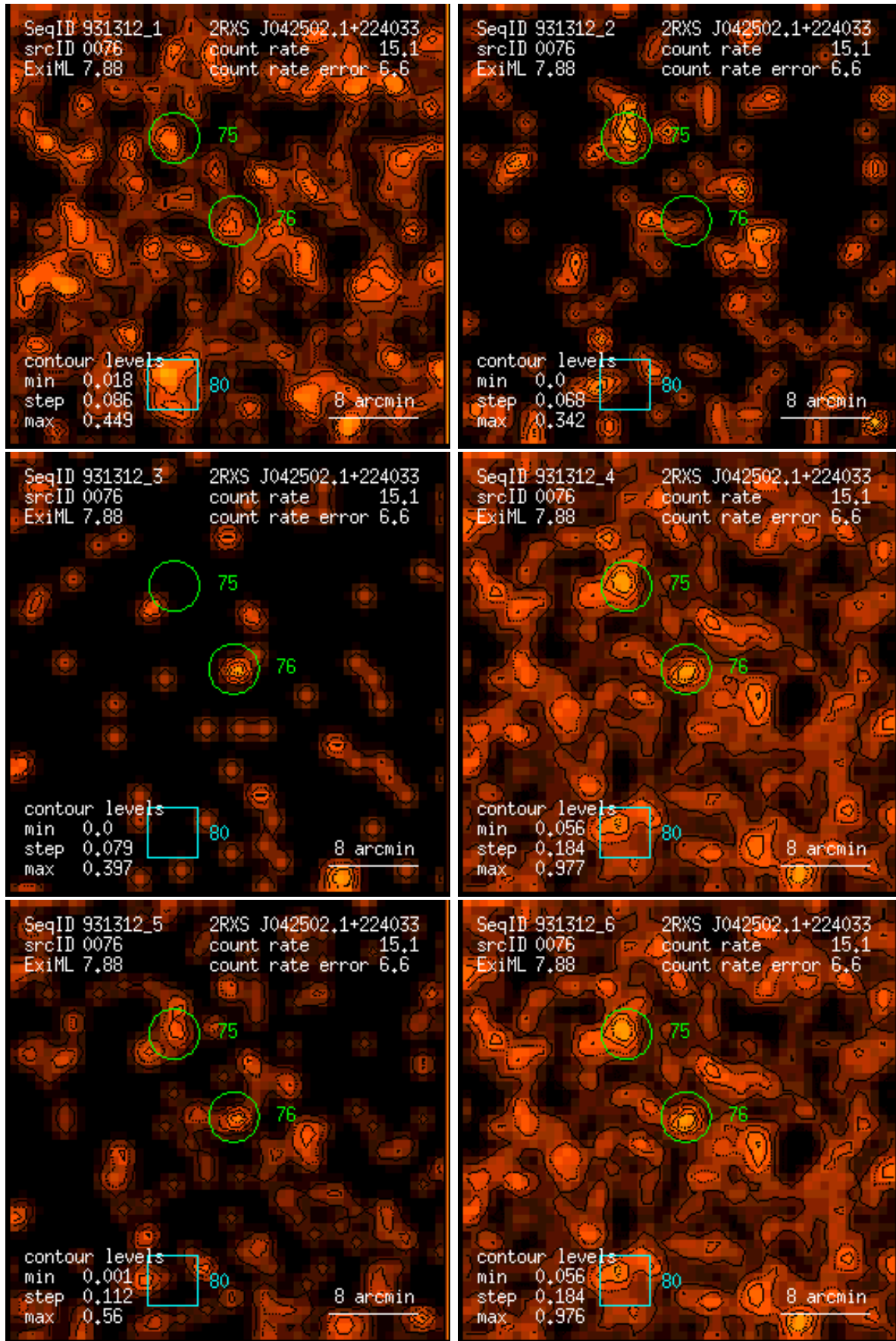
Figure 76: RASS 931312: detection 0076: band rate images, Gaussian filter: (1) PSPC channels 11 – 41, (2) 52 – 90, (3) 91 – 201, (4) 11 – 235, (5) 52 – 201, (6) 11 – 201. Broad band rates in counts/ks. Band rate contour levels in counts/ks/arcmin 2 .
