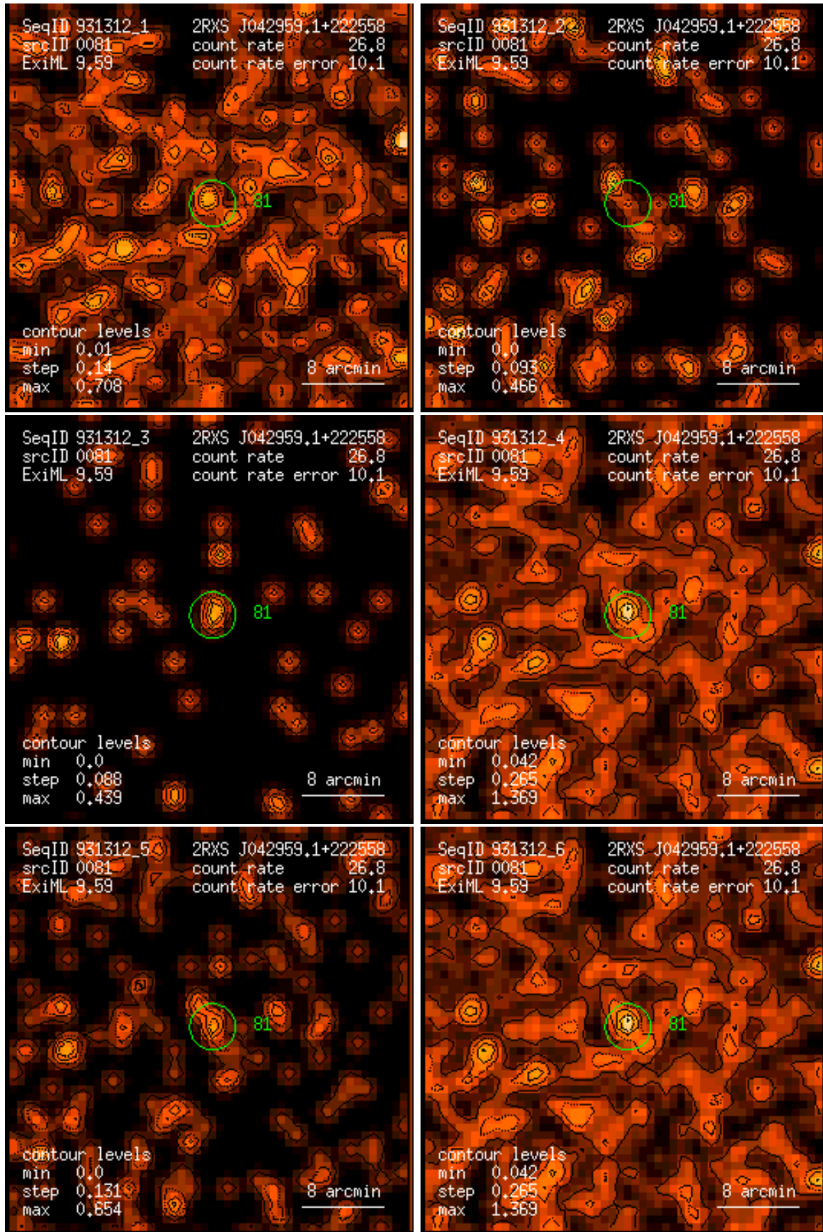
Figure 81: RASS 931312: detection 0081: band rate images, Gaussian filter: (1) PSPC channels 11 – 41, (2) 52 – 90, (3) 91 – 201, (4) 11 – 235, (5) 52 – 201, (6) 11 – 201. Broad band rates in counts/ks. Band rate contour levels in counts/ks/arcmin 2 .
