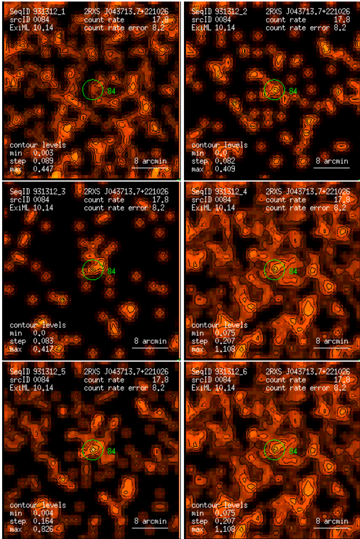
Figure 84: RASS 931312: detection 0084: band rate images, Gaussian filter: (1) PSPC channels 11 – 41, (2) 52 – 90, (3) 91 – 201, (4) 11 – 235, (5) 52 – 201, (6) 11 – 201. Broad band rates in counts/ks. Band rate contour levels in counts/ks/arcmin 2 .
