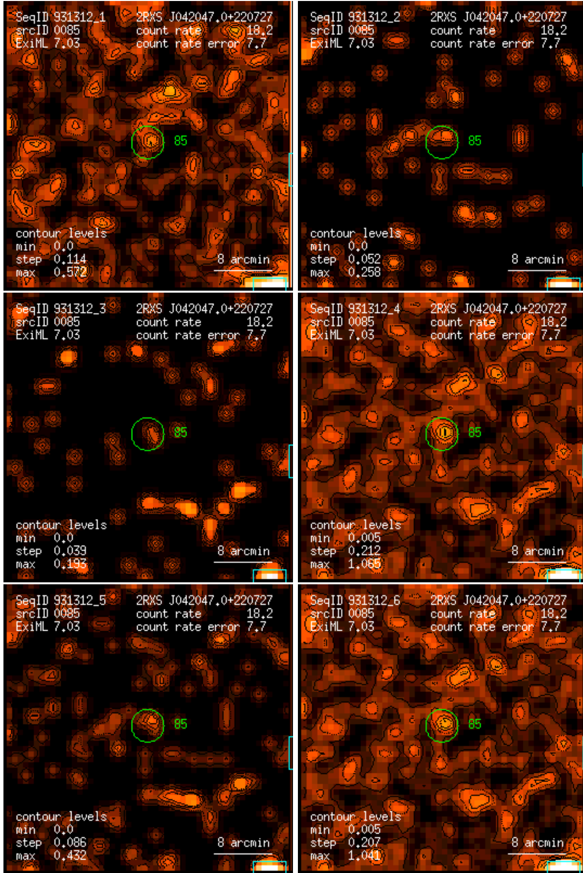
Figure 85: RASS 931312: detection 0085: band rate images, Gaussian filter: (1) PSPC channels 11 – 41, (2) 52 – 90, (3) 91 – 201, (4) 11 – 235, (5) 52 – 201, (6) 11 – 201. Broad band rates in counts/ks. Band rate contour levels in counts/ks/arcmin 2 .
