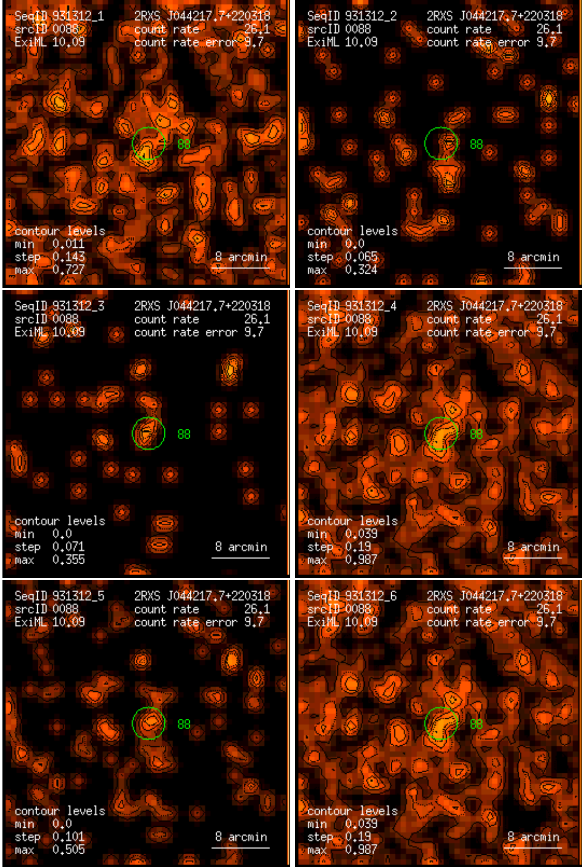
Figure 88: RASS 931312: detection 0088: band rate images, Gaussian filter: (1) PSPC channels 11 – 41, (2) 52 – 90, (3) 91 – 201, (4) 11 – 235, (5) 52 – 201, (6) 11 – 201. Broad band rates in counts/ks. Band rate contour levels in counts/ks/arcmin 2 .
