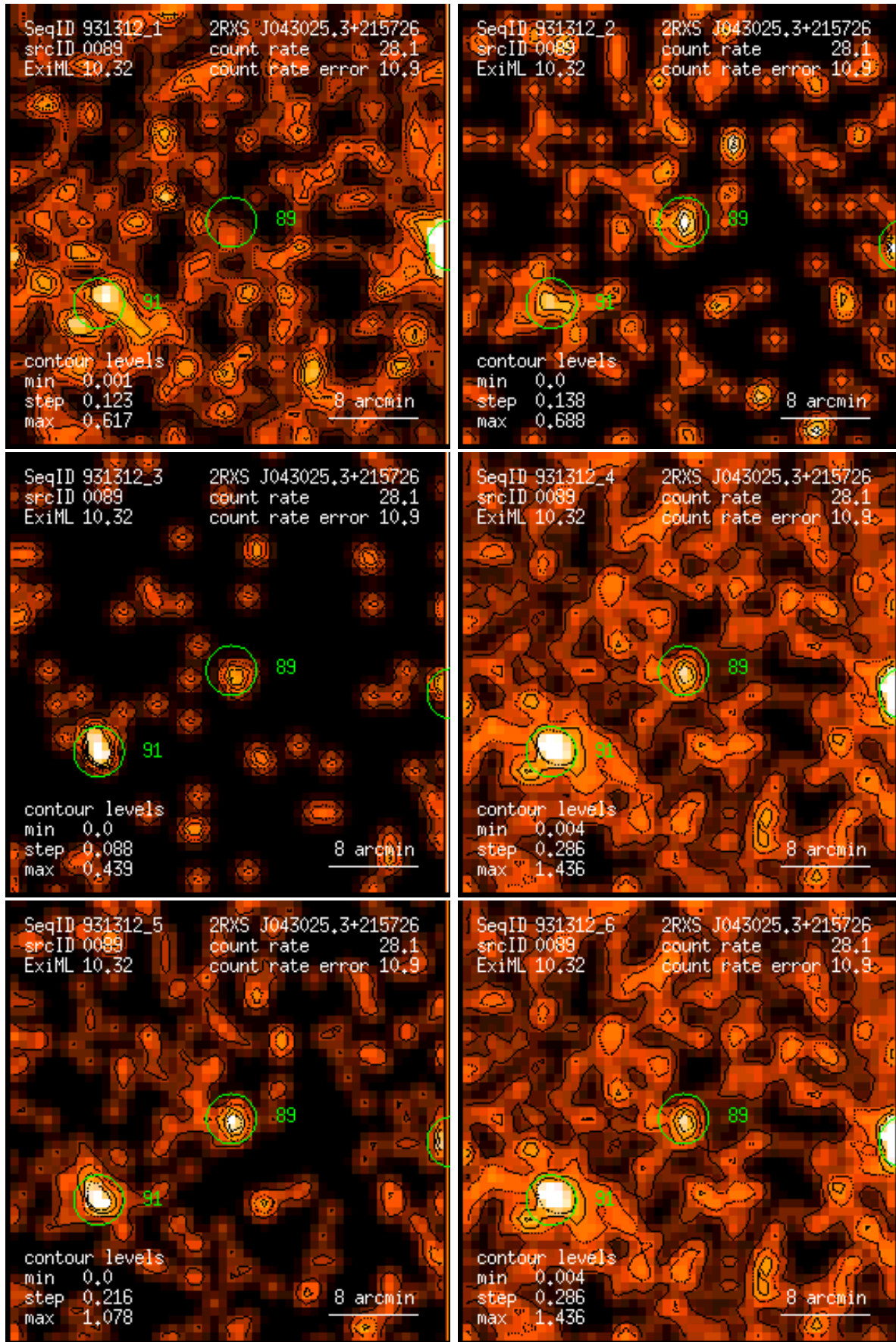
Figure 89: RASS 931312: detection 0089: band rate images, Gaussian filter: (1) PSPC channels 11 – 41, (2) 52 – 90, (3) 91 – 201, (4) 11 – 235, (5) 52 – 201, (6) 11 – 201. Broad band rates in counts/ks. Band rate contour levels in counts/ks/arcmin 2 .
