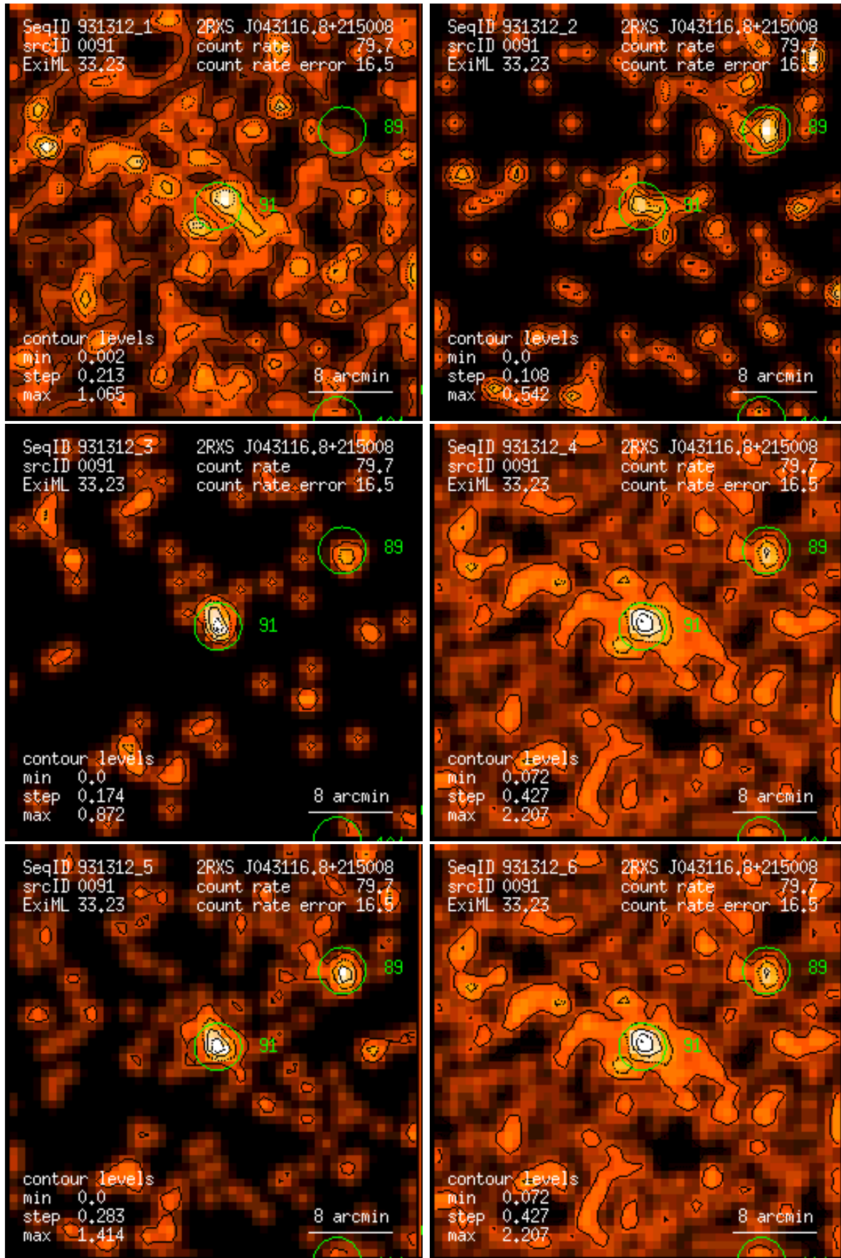
Figure 91: RASS 931312: detection 0091: band rate images, Gaussian filter: (1) PSPC channels 11 – 41, (2) 52 – 90, (3) 91 – 201, (4) 11 – 235, (5) 52 – 201, (6) 11 – 201. Broad band rates in counts/ks. Band rate contour levels in counts/ks/arcmin 2 .
