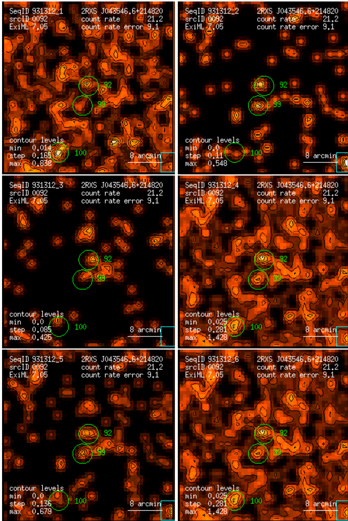
Figure 92: RASS 931312: detection 0092: band rate images, Gaussian filter: (1) PSPC channels 11 – 41, (2) 52 – 90, (3) 91 – 201, (4) 11 – 235, (5) 52 – 201, (6) 11 – 201. Broad band rates in counts/ks. Band rate contour levels in counts/ks/arcmin 2 .
