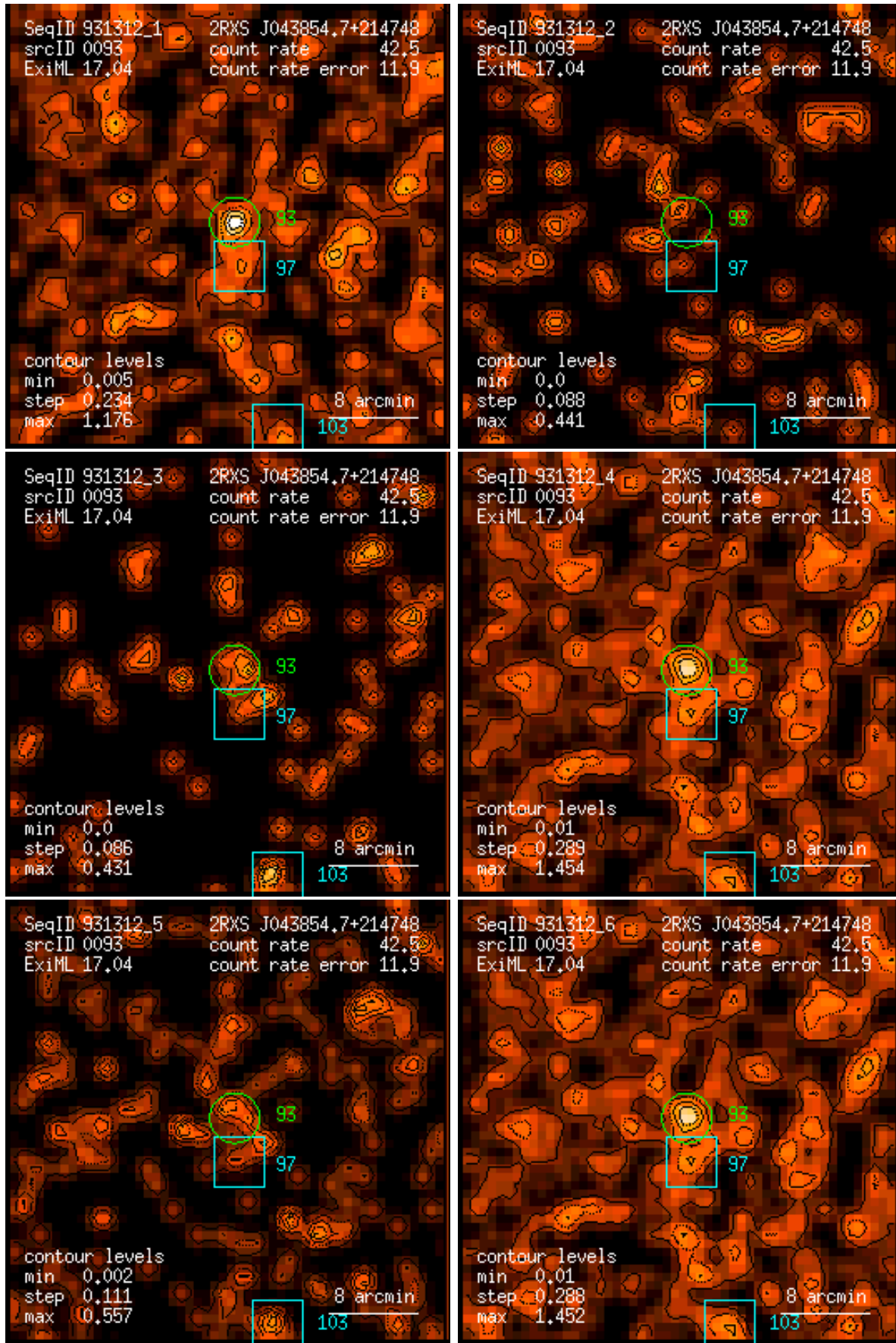
Figure 93: RASS 931312: detection 0093: band rate images, Gaussian filter: (1) PSPC channels 11 – 41, (2) 52 – 90, (3) 91 – 201, (4) 11 – 235, (5) 52 – 201, (6) 11 – 201. Broad band rates in counts/ks. Band rate contour levels in counts/ks/arcmin 2 .
