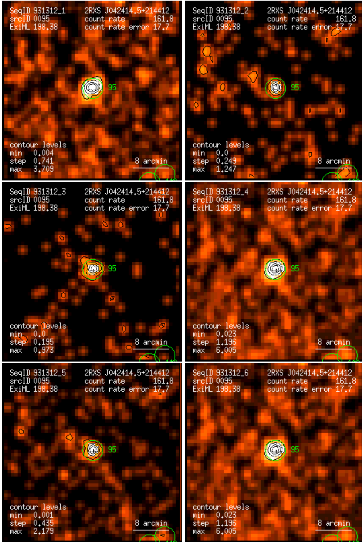
Figure 95: RASS 931312: detection 0095: band rate images, Gaussian filter: (1) PSPC channels 11 – 41, (2) 52 – 90, (3) 91 – 201, (4) 11 – 235, (5) 52 – 201, (6) 11 – 201. Broad band rates in counts/ks. Band rate contour levels in counts/ks/arcmin 2 .
